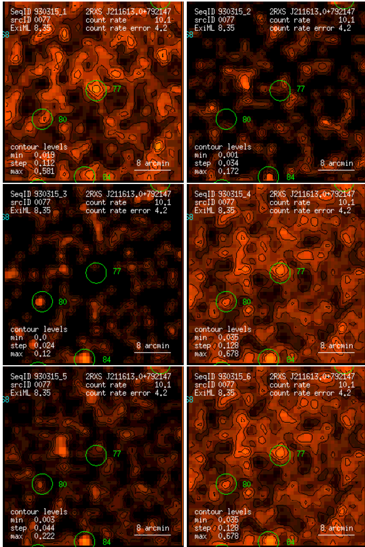
Figure 77: RASS 930315: detection 0077: band rate images, Gaussian filter: (1) PSPC channels 11 – 41, (2) 52 – 90, (3) 91 – 201, (4) 11 – 235, (5) 52 – 201, (6) 11 – 201. Broad band rates in counts/ks. Band rate contour levels in counts/ks/arcmin 2 .
