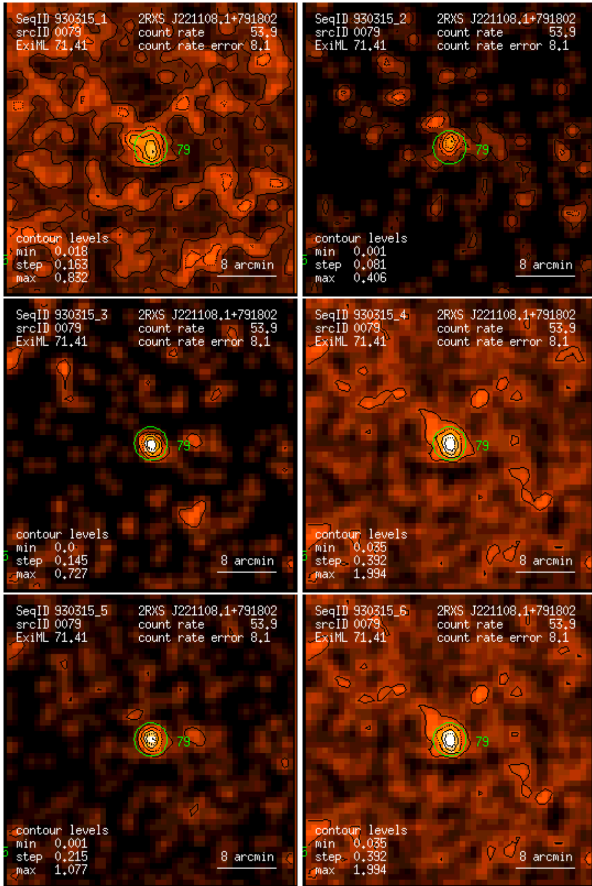
Figure 79: RASS 930315: detection 0079: band rate images, Gaussian filter: (1) PSPC channels 11 – 41, (2) 52 – 90, (3) 91 – 201, (4) 11 – 235, (5) 52 – 201, (6) 11 – 201. Broad band rates in counts/ks. Band rate contour levels in counts/ks/arcmin 2 .
