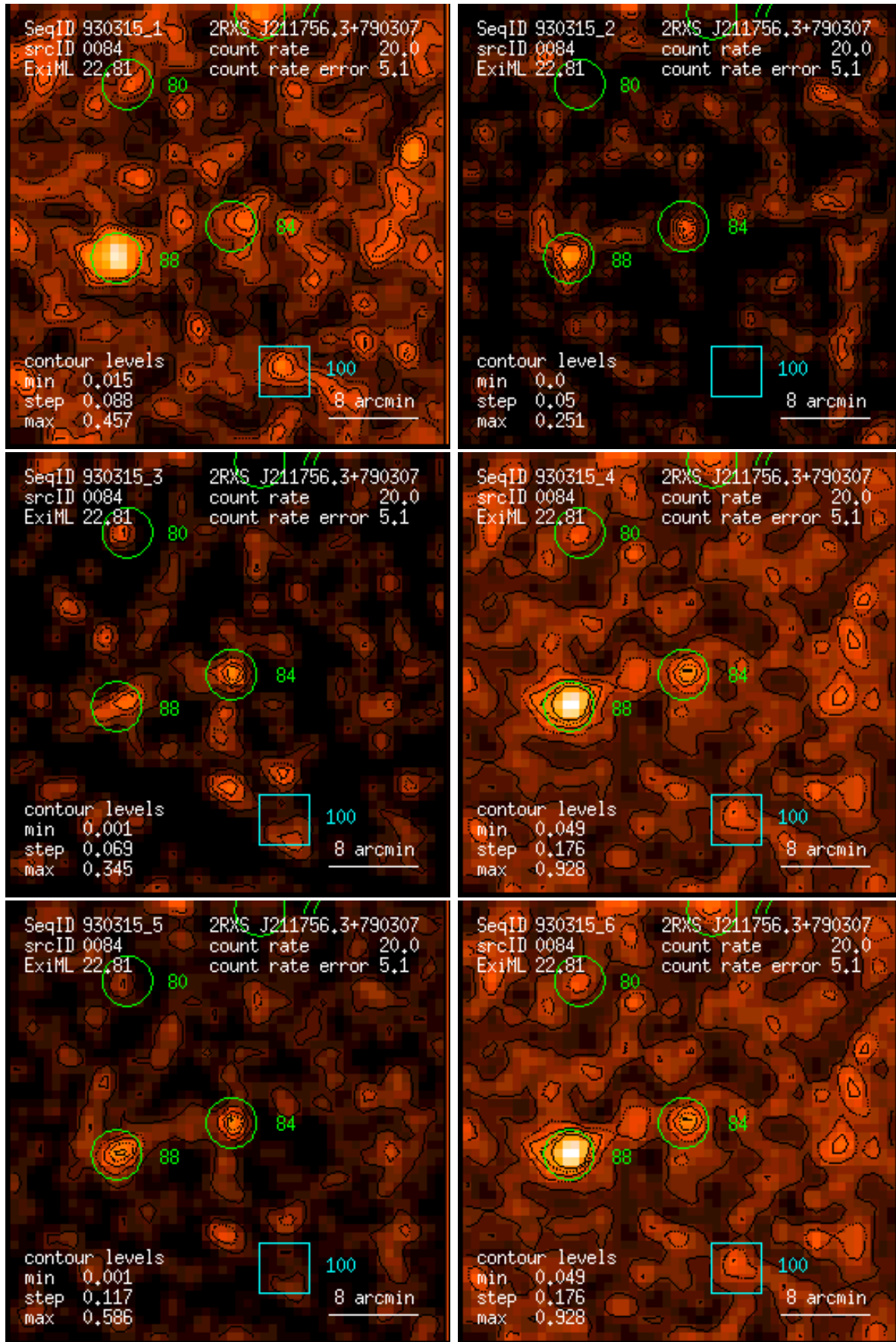
Figure 84: RASS 930315: detection 0084: band rate images, Gaussian filter: (1) PSPC channels 11 – 41, (2) 52 – 90, (3) 91 – 201, (4) 11 – 235, (5) 52 – 201, (6) 11 – 201. Broad band rates in counts/ks. Band rate contour levels in counts/ks/arcmin 2 .
