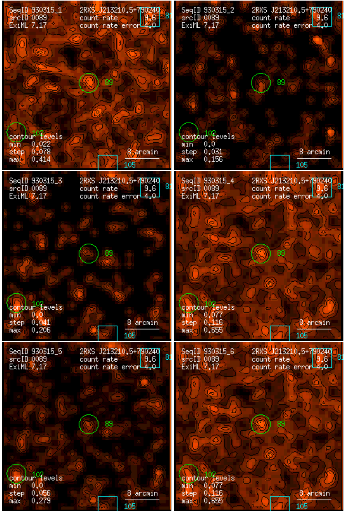
Figure 89: RASS 930315: detection 0089: band rate images, Gaussian filter: (1) PSPC channels 11 – 41, (2) 52 – 90, (3) 91 – 201, (4) 11 – 235, (5) 52 – 201, (6) 11 – 201. Broad band rates in counts/ks. Band rate contour levels in counts/ks/arcmin 2 .
