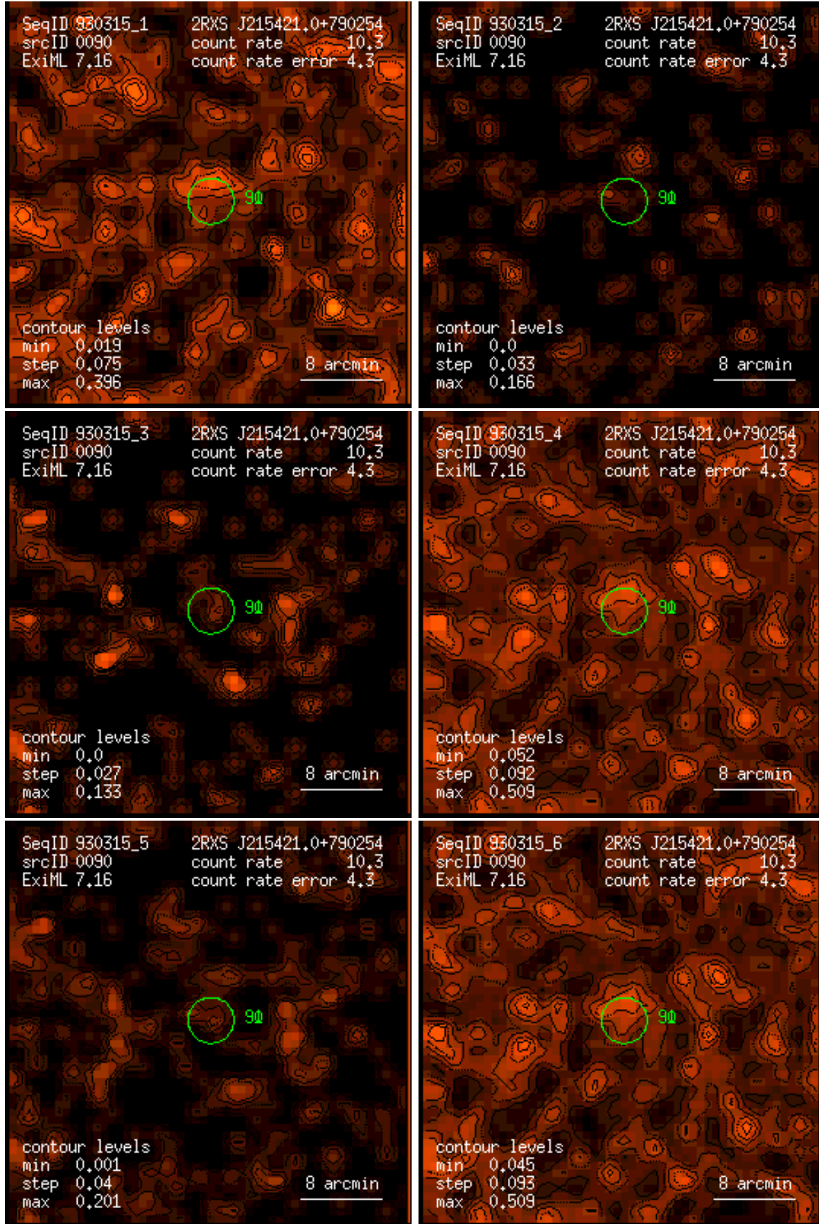
Figure 90: RASS 930315: detection 0090: band rate images, Gaussian filter: (1) PSPC channels 11 – 41, (2) 52 – 90, (3) 91 – 201, (4) 11 – 235, (5) 52 – 201, (6) 11 – 201. Broad band rates in counts/ks. Band rate contour levels in counts/ks/arcmin 2 .
