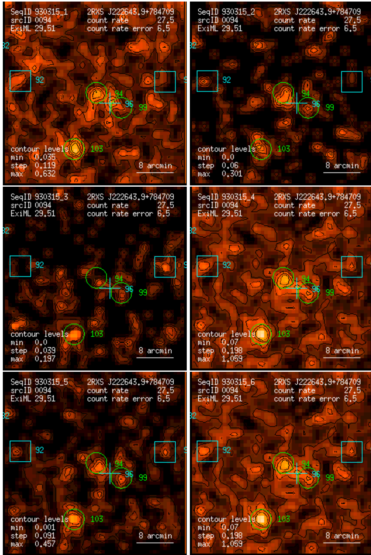
Figure 94: RASS 930315: detection 0094: band rate images, Gaussian filter: (1) PSPC channels 11 – 41, (2) 52 – 90, (3) 91 – 201, (4) 11 – 235, (5) 52 – 201, (6) 11 – 201. Broad band rates in counts/ks. Band rate contour levels in counts/ks/arcmin 2 .
