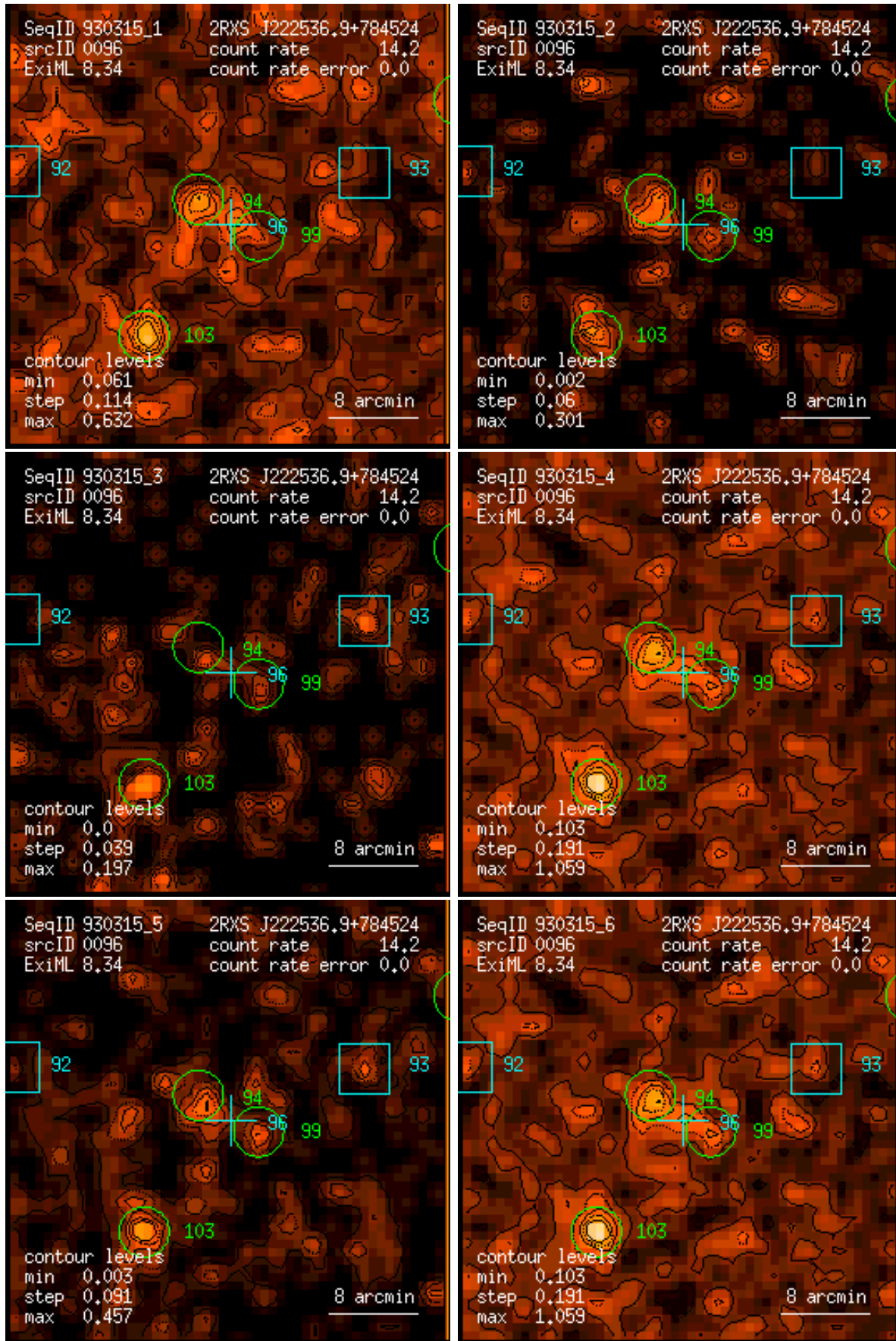
Figure 96: RASS 930315: detection 0096: band rate images, Gaussian filter: (1) PSPC channels 11 – 41, (2) 52 – 90, (3) 91 – 201, (4) 11 – 235, (5) 52 – 201, (6) 11 – 201. Broad band rates in counts/ks. Band rate contour levels in counts/ks/arcmin 2 .
