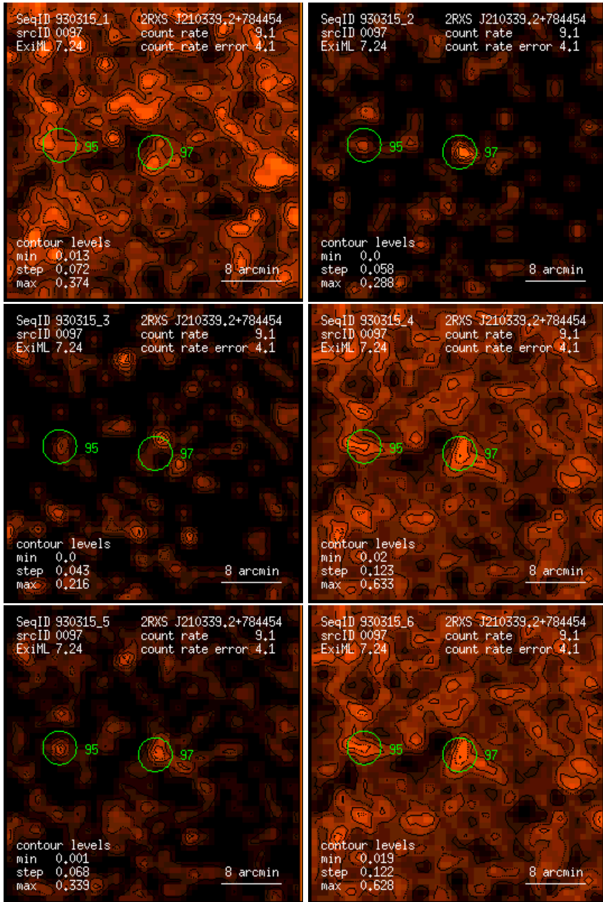
Figure 97: RASS 930315: detection 0097: band rate images, Gaussian filter: (1) PSPC channels 11 – 41, (2) 52 – 90, (3) 91 – 201, (4) 11 – 235, (5) 52 – 201, (6) 11 – 201. Broad band rates in counts/ks. Band rate contour levels in counts/ks/arcmin 2 .
