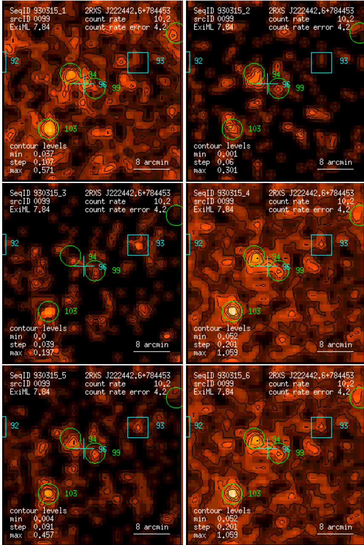
Figure 99: RASS 930315: detection 0099: band rate images, Gaussian filter: (1) PSPC channels 11 – 41, (2) 52 – 90, (3) 91 – 201, (4) 11 – 235, (5) 52 – 201, (6) 11 – 201. Broad band rates in counts/ks. Band rate contour levels in counts/ks/arcmin 2 .
