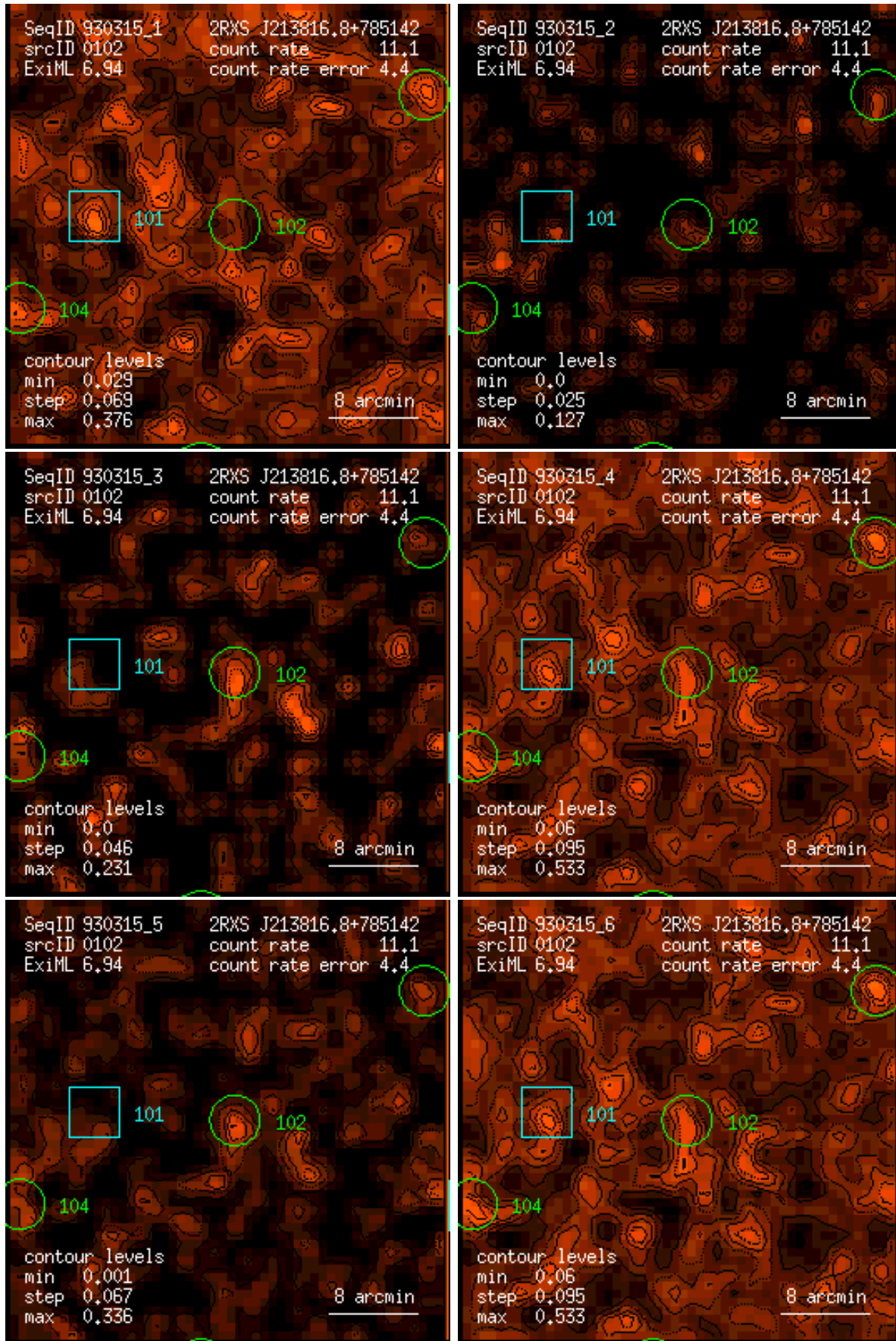
Figure 102: RASS 930315: detection 0102: band rate images, Gaussian filter: (1) PSPC channels 11 – 41, (2) 52 – 90, (3) 91 – 201, (4) 11 – 235, (5) 52 – 201, (6) 11 – 201. Broad band rates in counts/ks. Band rate contour levels in counts/ks/arcmin 2 .
