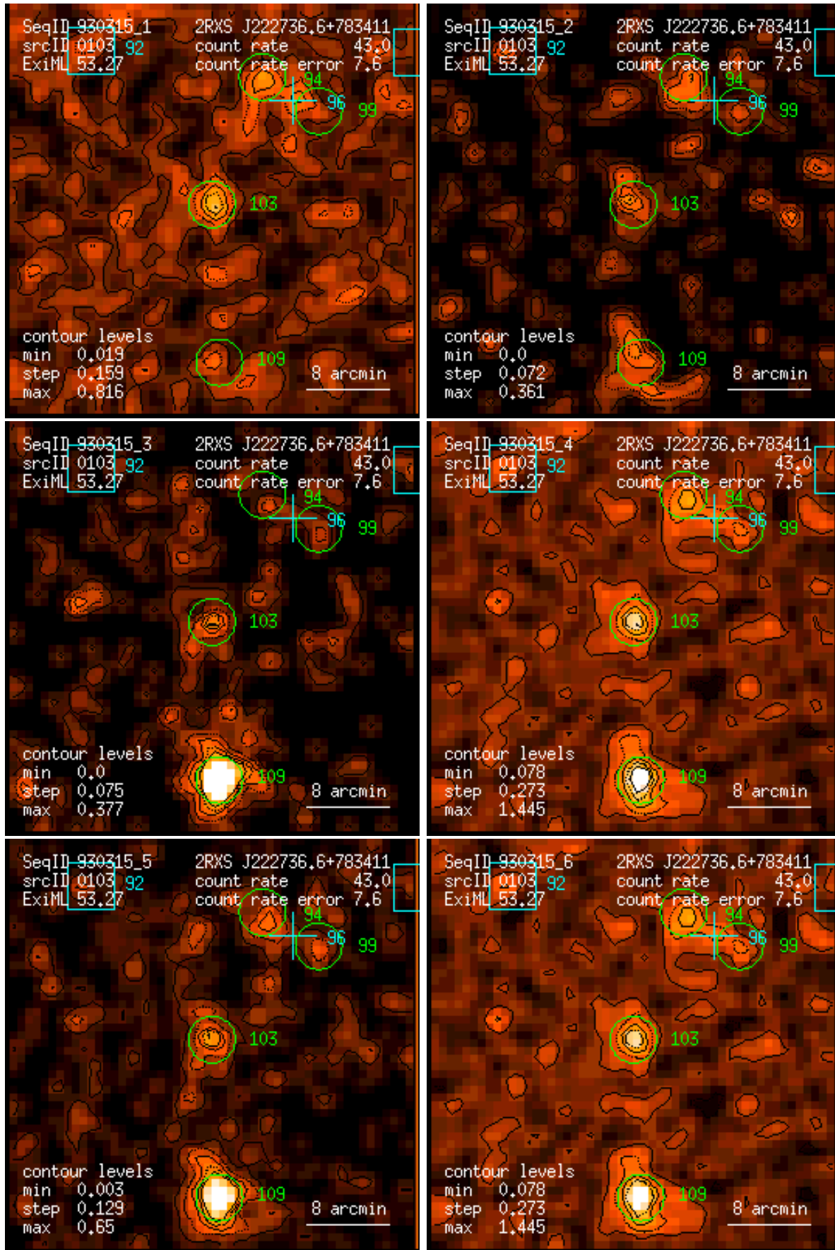
Figure 103: RASS 930315: detection 0103: band rate images, Gaussian filter: (1) PSPC channels 11 – 41, (2) 52 – 90, (3) 91 – 201, (4) 11 – 235, (5) 52 – 201, (6) 11 – 201. Broad band rates in counts/ks. Band rate contour levels in counts/ks/arcmin 2 .
