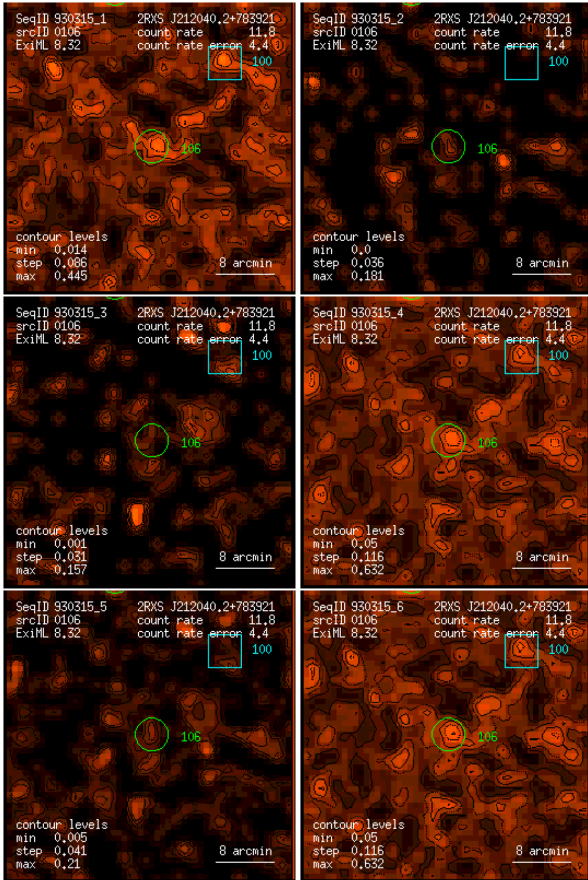
Figure 106: RASS 930315: detection 0106: band rate images, Gaussian filter: (1) PSPC channels 11 – 41, (2) 52 – 90, (3) 91 – 201, (4) 11 – 235, (5) 52 – 201, (6) 11 – 201. Broad band rates in counts/ks. Band rate contour levels in counts/ks/arcmin 2 .
