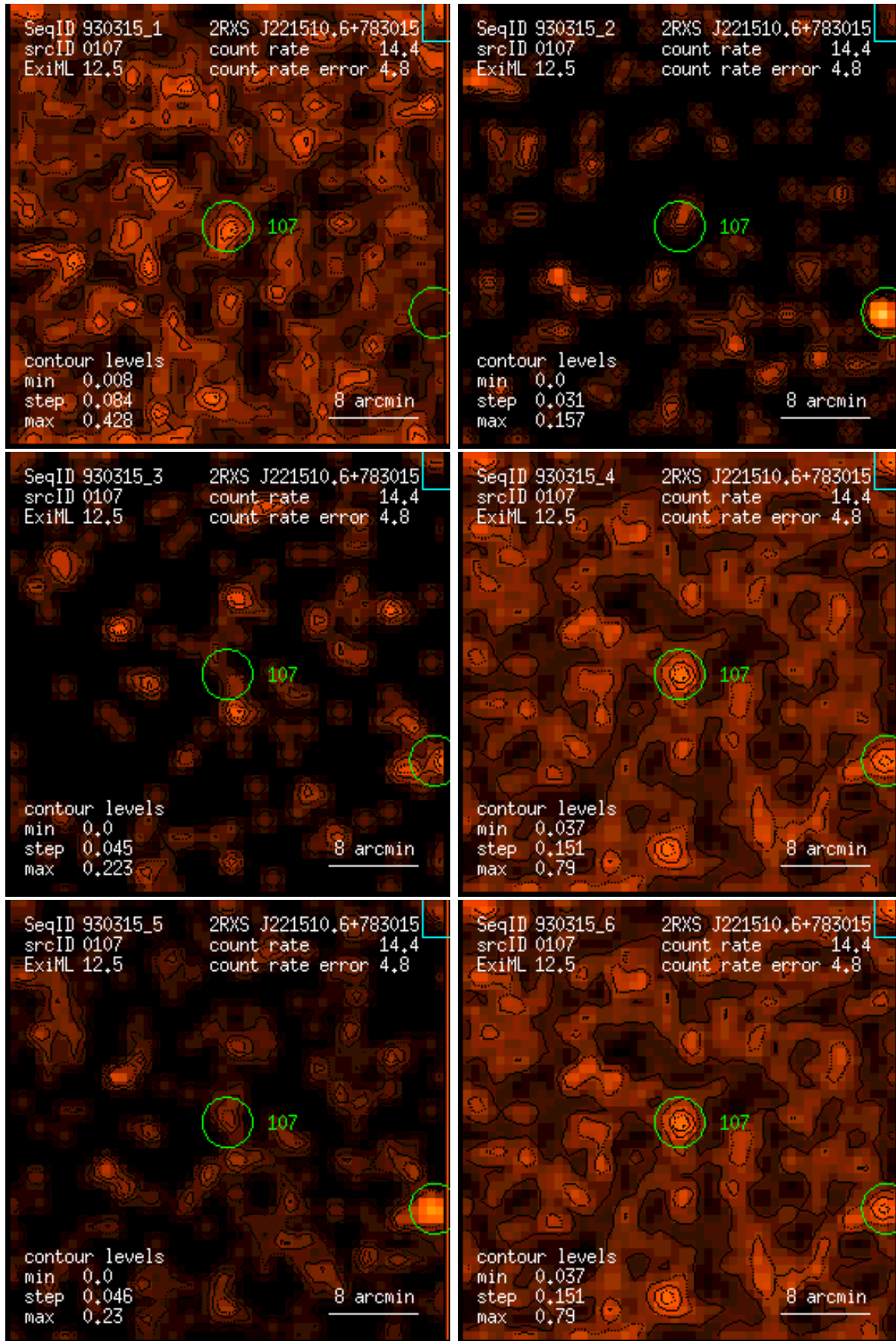
Figure 107: RASS 930315: detection 0107: band rate images, Gaussian filter: (1) PSPC channels 11 – 41, (2) 52 – 90, (3) 91 – 201, (4) 11 – 235, (5) 52 – 201, (6) 11 – 201. Broad band rates in counts/ks. Band rate contour levels in counts/ks/arcmin 2 .
