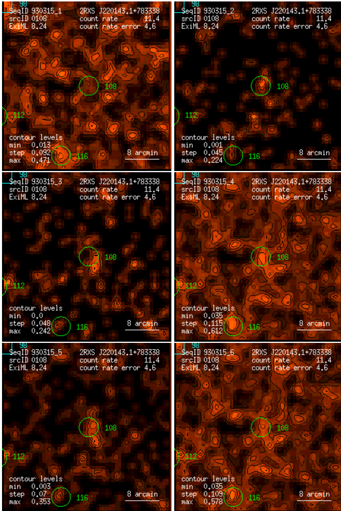
Figure 108: RASS 930315: detection 0108: band rate images, Gaussian filter: (1) PSPC channels 11 – 41, (2) 52 – 90, (3) 91 – 201, (4) 11 – 235, (5) 52 – 201, (6) 11 – 201. Broad band rates in counts/ks. Band rate contour levels in counts/ks/arcmin 2 .
