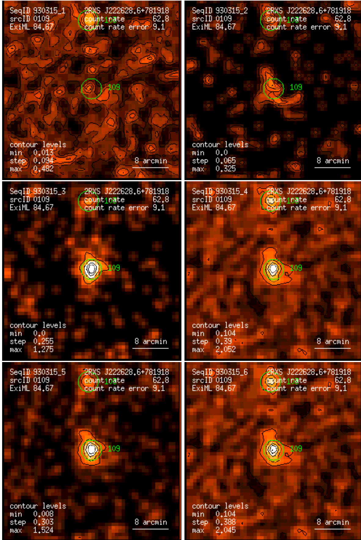
Figure 109: RASS 930315: detection 0109: band rate images, Gaussian filter: (1) PSPC channels 11 – 41, (2) 52 – 90, (3) 91 – 201, (4) 11 – 235, (5) 52 – 201, (6) 11 – 201. Broad band rates in counts/ks. Band rate contour levels in counts/ks/arcmin 2 .
