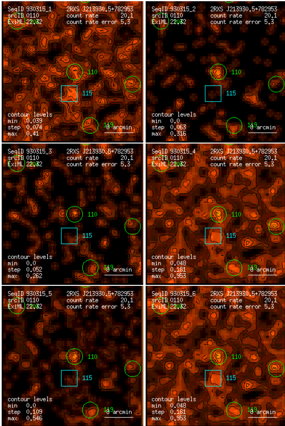
Figure 110: RASS 930315: detection 0110: band rate images, Gaussian filter: (1) PSPC channels 11 – 41, (2) 52 – 90, (3) 91 – 201, (4) 11 – 235, (5) 52 – 201, (6) 11 – 201. Broad band rates in counts/ks. Band rate contour levels in counts/ks/arcmin 2 .
