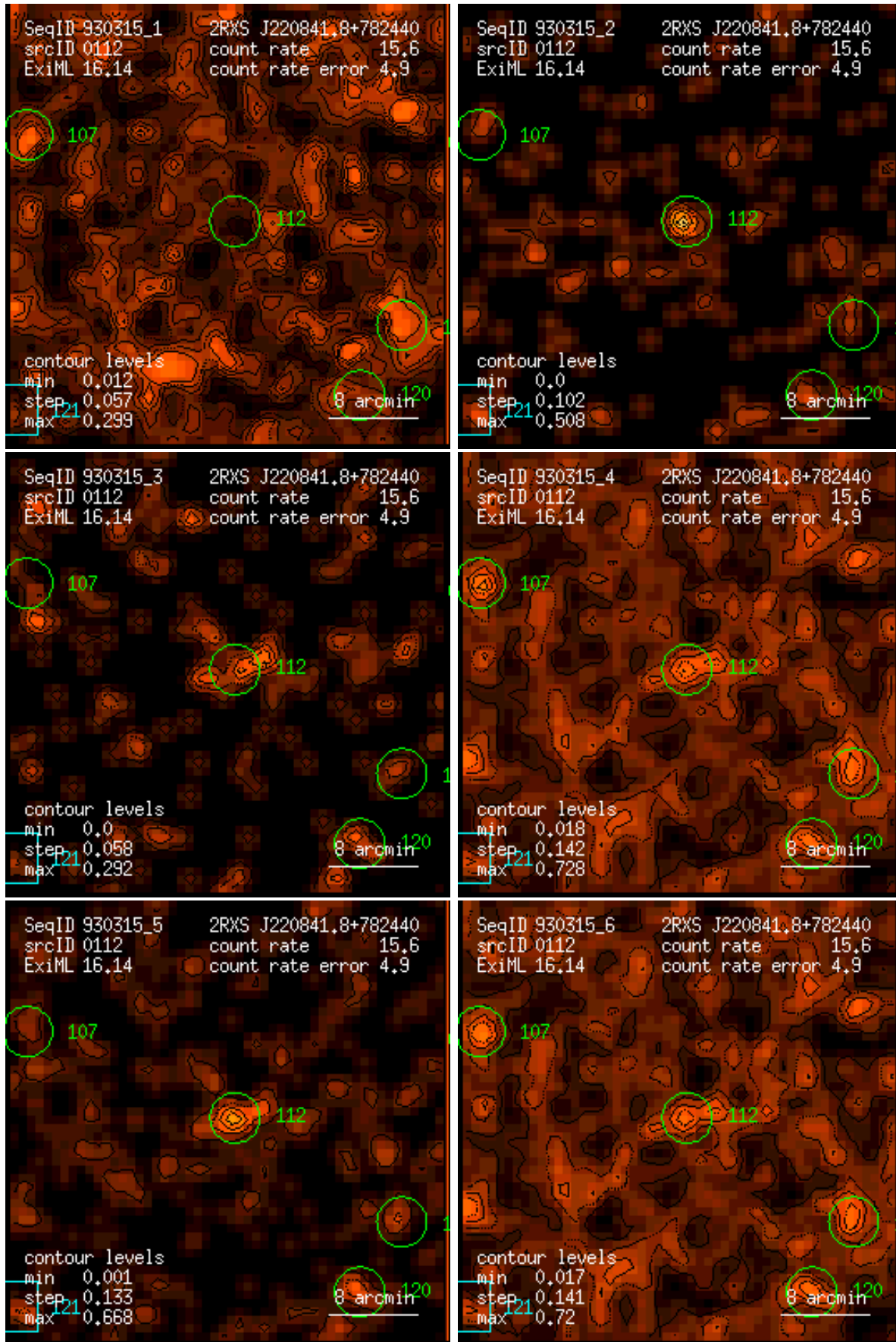
Figure 112: RASS 930315: detection 0112: band rate images, Gaussian filter: (1) PSPC channels 11 – 41, (2) 52 – 90, (3) 91 – 201, (4) 11 – 235, (5) 52 – 201, (6) 11 – 201. Broad band rates in counts/ks. Band rate contour levels in counts/ks/arcmin 2 .
