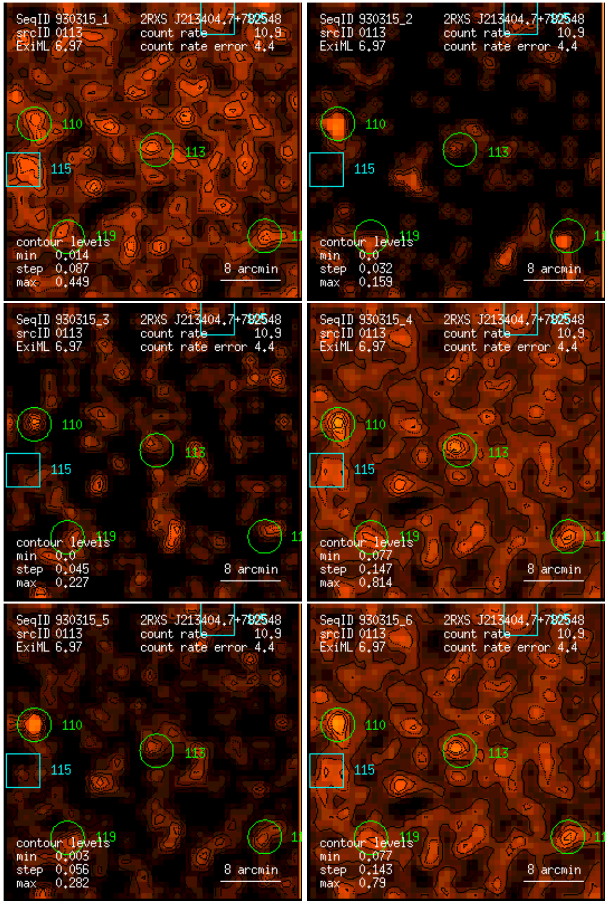
Figure 113: RASS 930315: detection 0113: band rate images, Gaussian filter: (1) PSPC channels 11 – 41, (2) 52 – 90, (3) 91 – 201, (4) 11 – 235, (5) 52 – 201, (6) 11 – 201. Broad band rates in counts/ks. Band rate contour levels in counts/ks/arcmin 2 .
