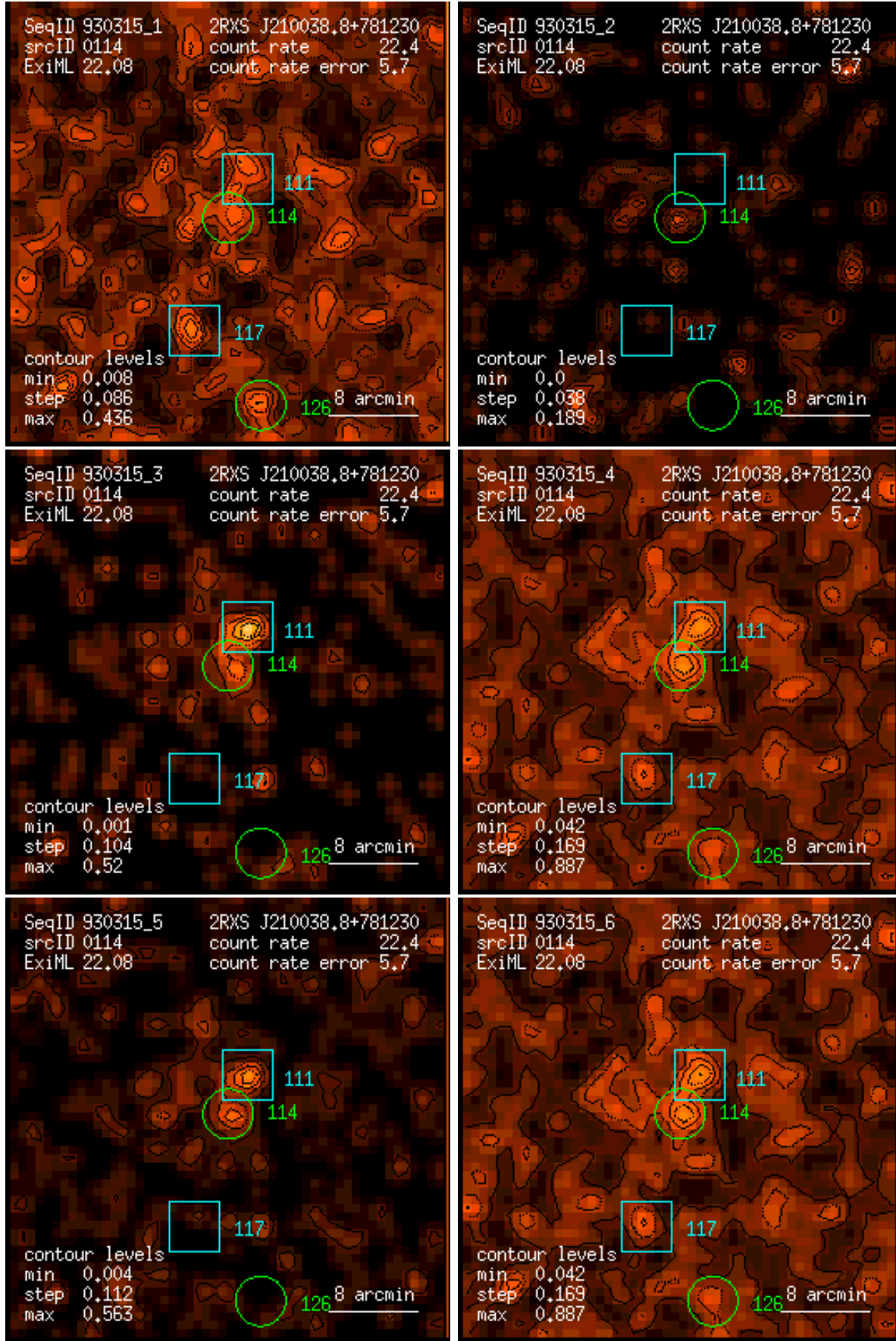
Figure 114: RASS 930315: detection 0114: band rate images, Gaussian filter: (1) PSPC channels 11 – 41, (2) 52 – 90, (3) 91 – 201, (4) 11 – 235, (5) 52 – 201, (6) 11 – 201. Broad band rates in counts/ks. Band rate contour levels in counts/ks/arcmin 2 .
