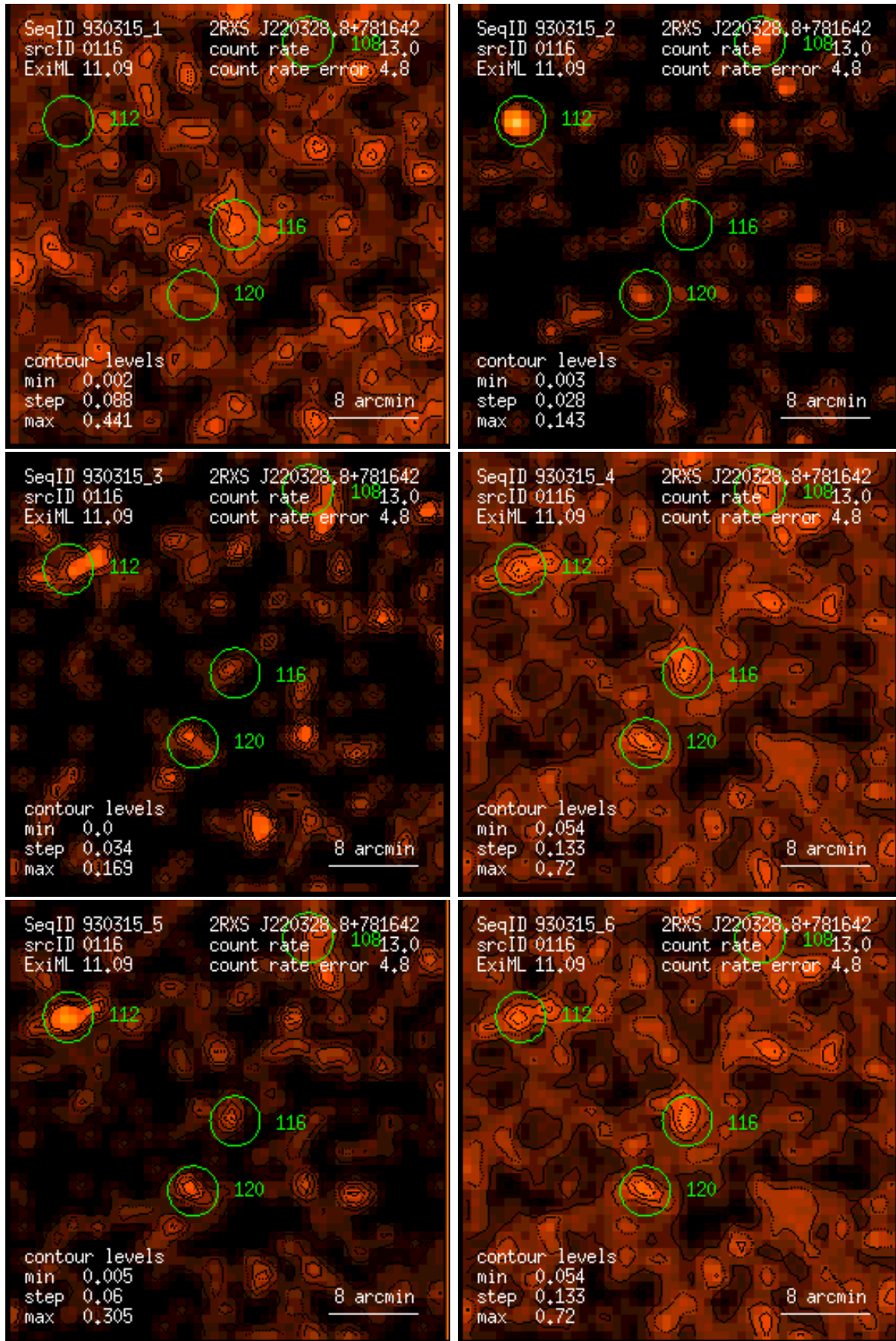
Figure 116: RASS 930315: detection 0116: band rate images, Gaussian filter: (1) PSPC channels 11 – 41, (2) 52 – 90, (3) 91 – 201, (4) 11 – 235, (5) 52 – 201, (6) 11 – 201. Broad band rates in counts/ks. Band rate contour levels in counts/ks/arcmin 2 .
