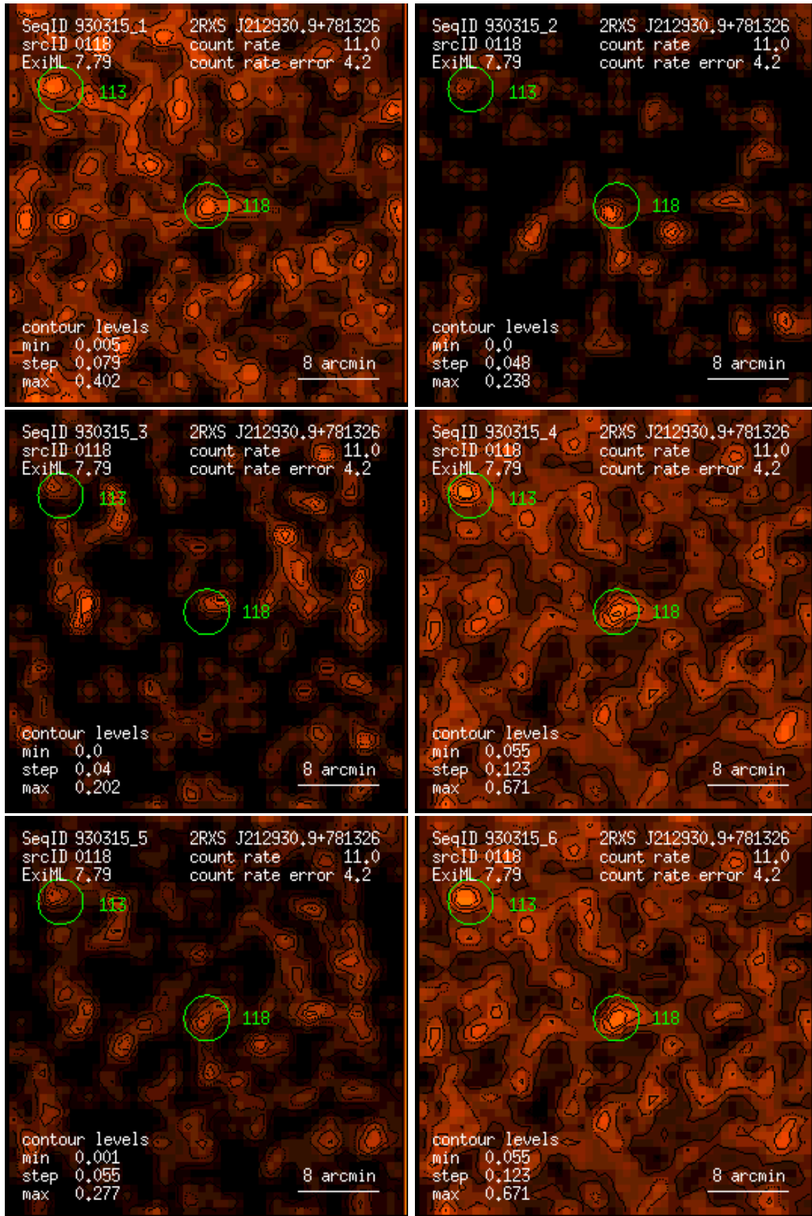
Figure 118: RASS 930315: detection 0118: band rate images, Gaussian filter: (1) PSPC channels 11 – 41, (2) 52 – 90, (3) 91 – 201, (4) 11 – 235, (5) 52 – 201, (6) 11 – 201. Broad band rates in counts/ks. Band rate contour levels in counts/ks/arcmin 2 .
