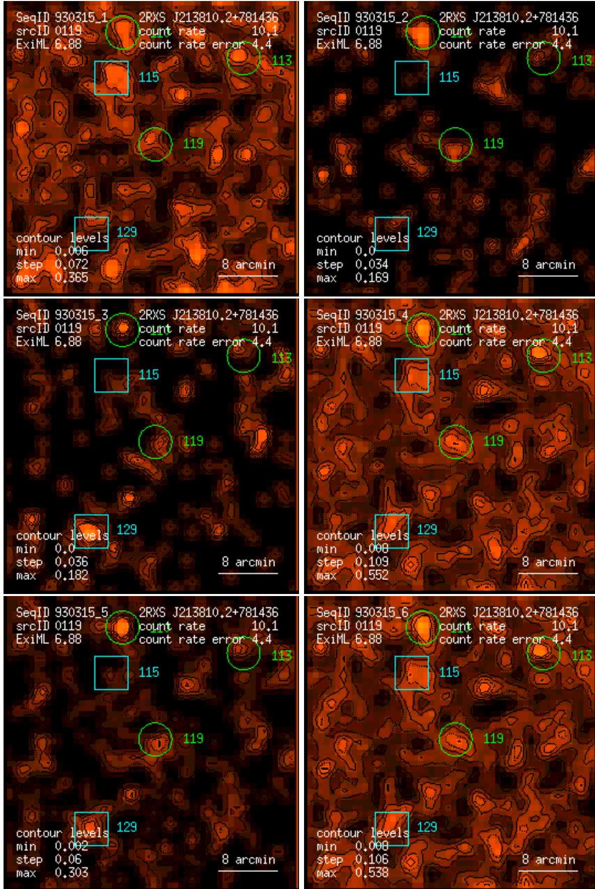
Figure 119: RASS 930315: detection 0119: band rate images, Gaussian filter: (1) PSPC channels 11 – 41, (2) 52 – 90, (3) 91 – 201, (4) 11 – 235, (5) 52 – 201, (6) 11 – 201. Broad band rates in counts/ks. Band rate contour levels in counts/ks/arcmin 2 .
