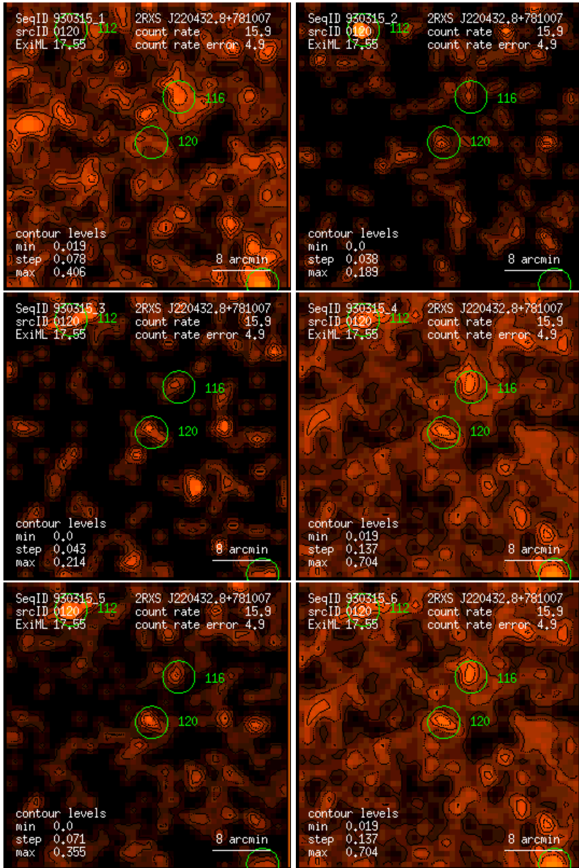
Figure 120: RASS 930315: detection 0120: band rate images, Gaussian filter: (1) PSPC channels 11 – 41, (2) 52 – 90, (3) 91 – 201, (4) 11 – 235, (5) 52 – 201, (6) 11 – 201. Broad band rates in counts/ks. Band rate contour levels in counts/ks/arcmin 2 .
