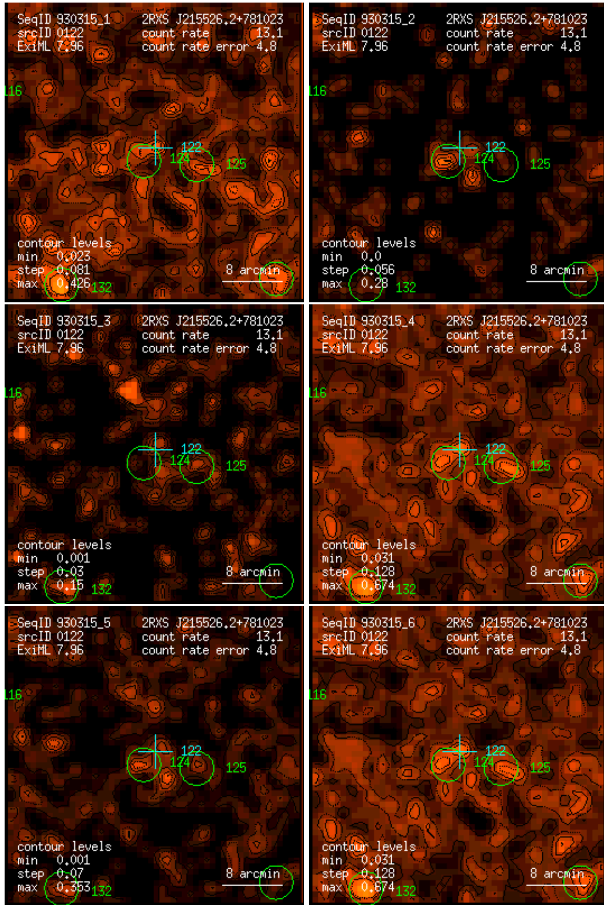
Figure 122: RASS 930315: detection 0122: band rate images, Gaussian filter: (1) PSPC channels 11 – 41, (2) 52 – 90, (3) 91 – 201, (4) 11 – 235, (5) 52 – 201, (6) 11 – 201. Broad band rates in counts/ks. Band rate contour levels in counts/ks/arcmin 2 .
