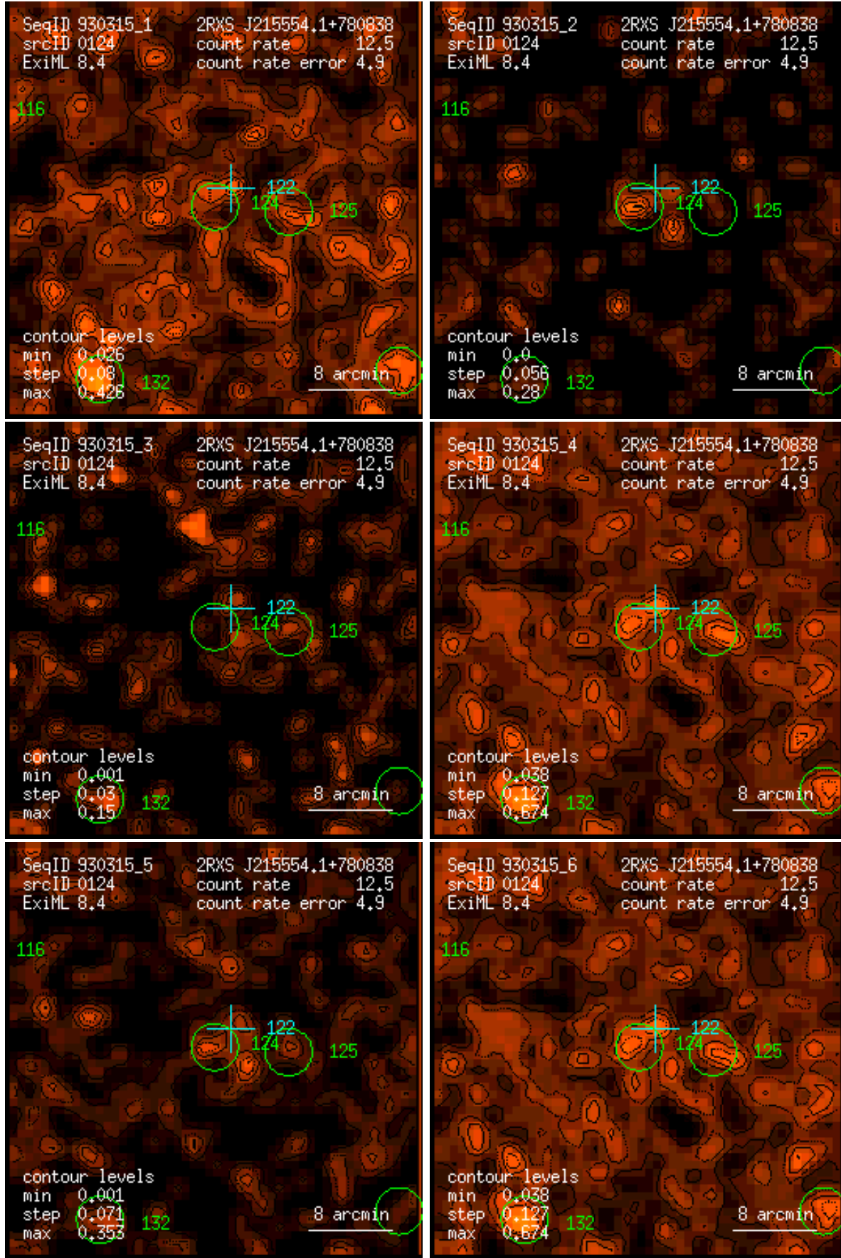
Figure 124: RASS 930315: detection 0124: band rate images, Gaussian filter: (1) PSPC channels 11 – 41, (2) 52 – 90, (3) 91 – 201, (4) 11 – 235, (5) 52 – 201, (6) 11 – 201. Broad band rates in counts/ks. Band rate contour levels in counts/ks/arcmin 2 .
