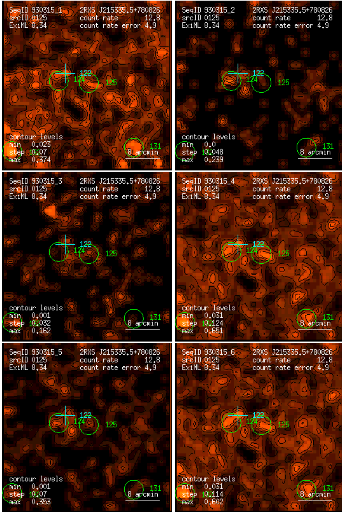
Figure 125: RASS 930315: detection 0125: band rate images, Gaussian filter: (1) PSPC channels 11 – 41, (2) 52 – 90, (3) 91 – 201, (4) 11 – 235, (5) 52 – 201, (6) 11 – 201. Broad band rates in counts/ks. Band rate contour levels in counts/ks/arcmin 2 .
