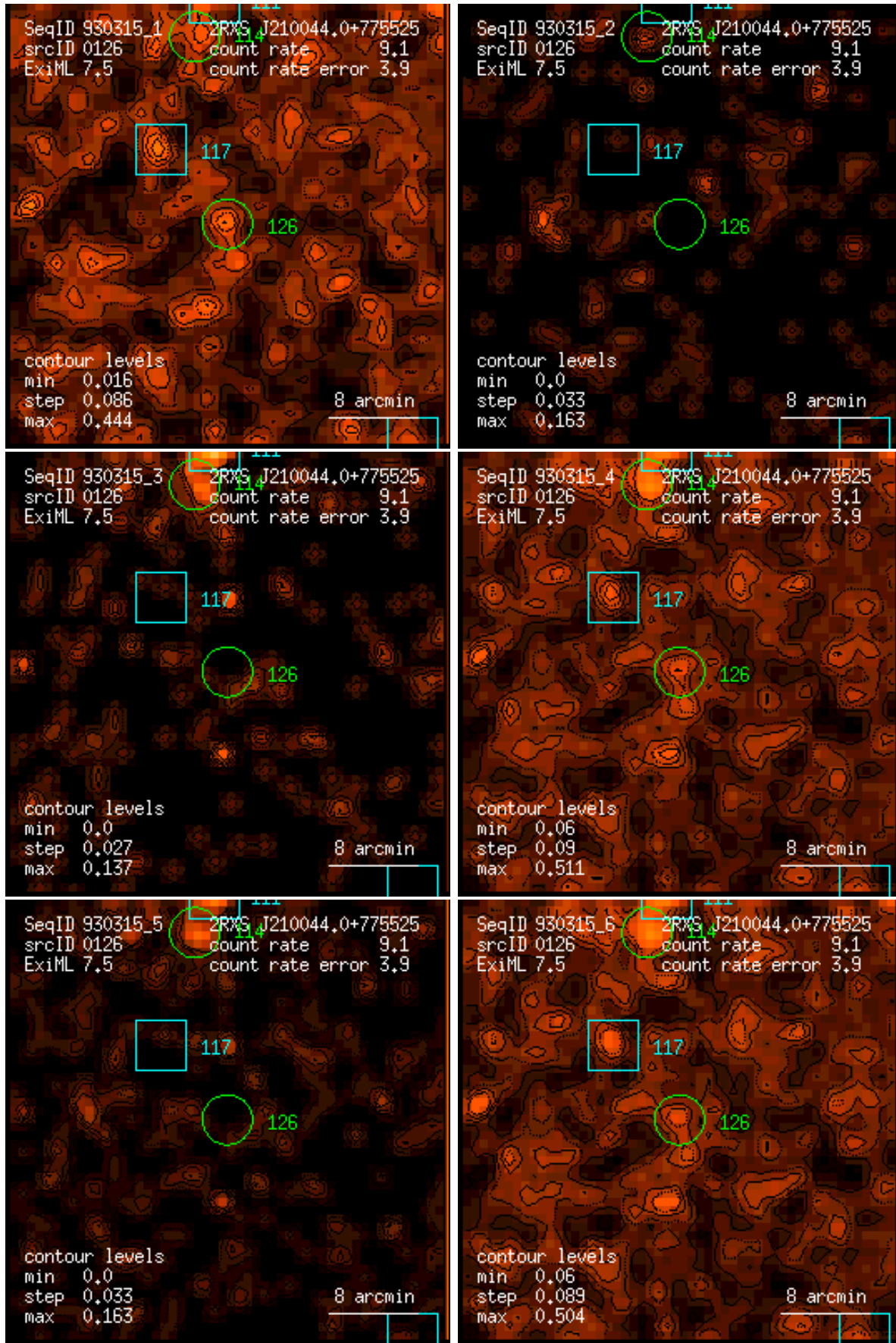
Figure 126: RASS 930315: detection 0126: band rate images, Gaussian filter: (1) PSPC channels 11 – 41, (2) 52 – 90, (3) 91 – 201, (4) 11 – 235, (5) 52 – 201, (6) 11 – 201. Broad band rates in counts/ks. Band rate contour levels in counts/ks/arcmin 2 .
