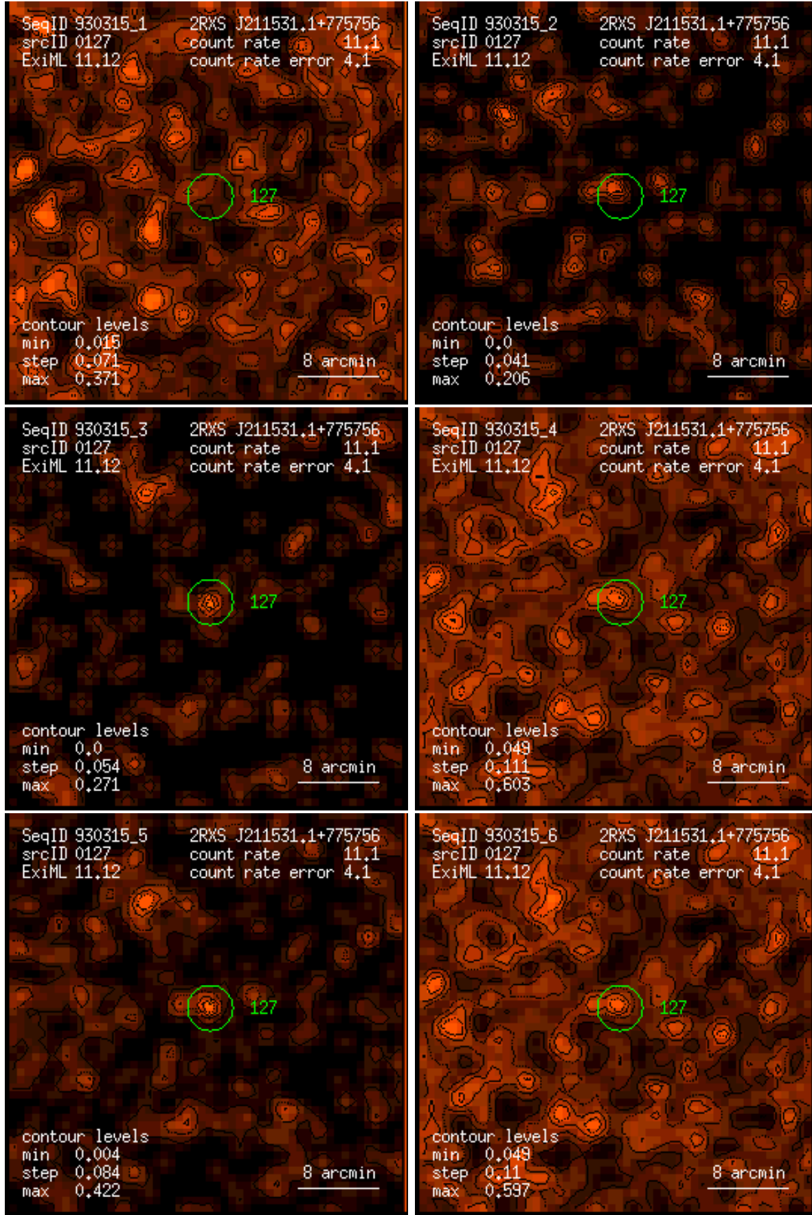
Figure 127: RASS 930315: detection 0127: band rate images, Gaussian filter: (1) PSPC channels 11 – 41, (2) 52 – 90, (3) 91 – 201, (4) 11 – 235, (5) 52 – 201, (6) 11 – 201. Broad band rates in counts/ks. Band rate contour levels in counts/ks/arcmin 2 .
