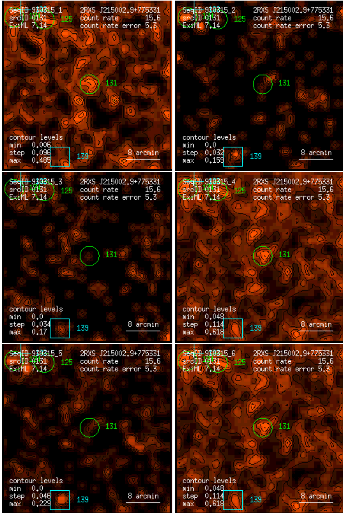
Figure 131: RASS 930315: detection 0131: band rate images, Gaussian filter: (1) PSPC channels 11 – 41, (2) 52 – 90, (3) 91 – 201, (4) 11 – 235, (5) 52 – 201, (6) 11 – 201. Broad band rates in counts/ks. Band rate contour levels in counts/ks/arcmin 2 .
