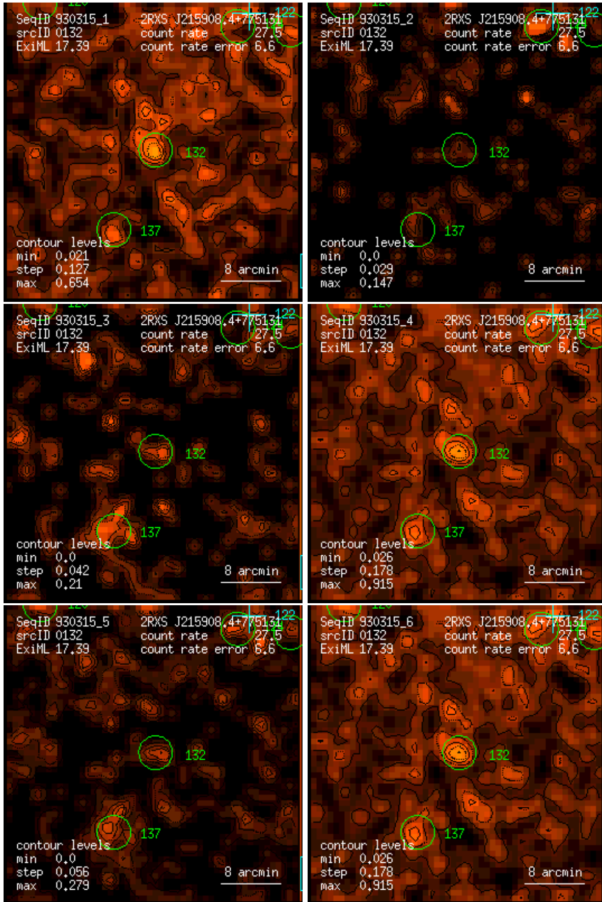
Figure 132: RASS 930315: detection 0132: band rate images, Gaussian filter: (1) PSPC channels 11 – 41, (2) 52 – 90, (3) 91 – 201, (4) 11 – 235, (5) 52 – 201, (6) 11 – 201. Broad band rates in counts/ks. Band rate contour levels in counts/ks/arcmin 2 .
