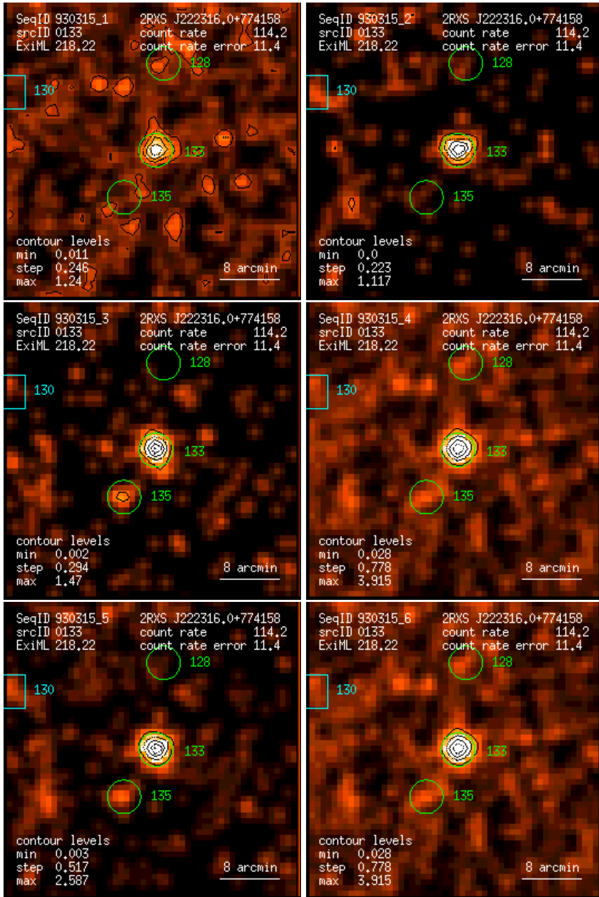
Figure 133: RASS 930315: detection 0133: band rate images, Gaussian filter: (1) PSPC channels 11 – 41, (2) 52 – 90, (3) 91 – 201, (4) 11 – 235, (5) 52 – 201, (6) 11 – 201. Broad band rates in counts/ks. Band rate contour levels in counts/ks/arcmin 2 .
