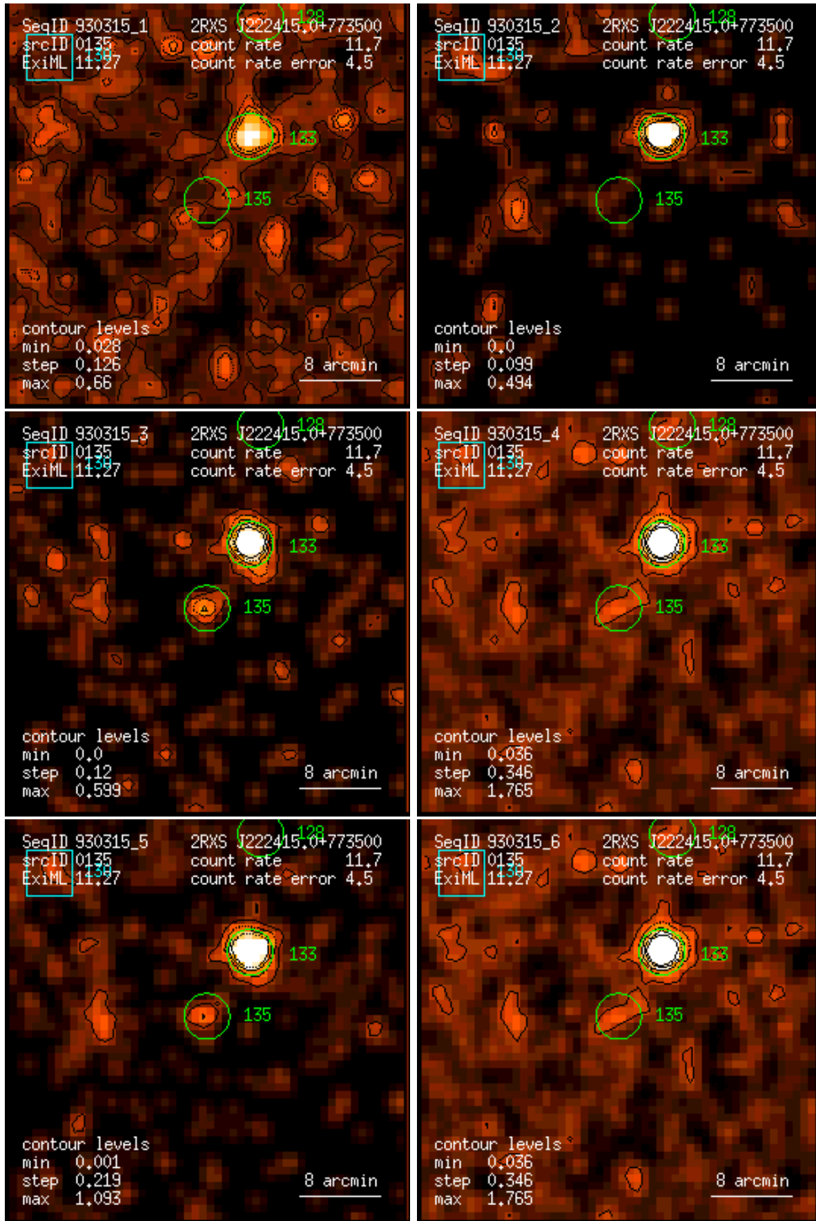
Figure 135: RASS 930315: detection 0135: band rate images, Gaussian filter: (1) PSPC channels 11 – 41, (2) 52 – 90, (3) 91 – 201, (4) 11 – 235, (5) 52 – 201, (6) 11 – 201. Broad band rates in counts/ks. Band rate contour levels in counts/ks/arcmin 2 .
