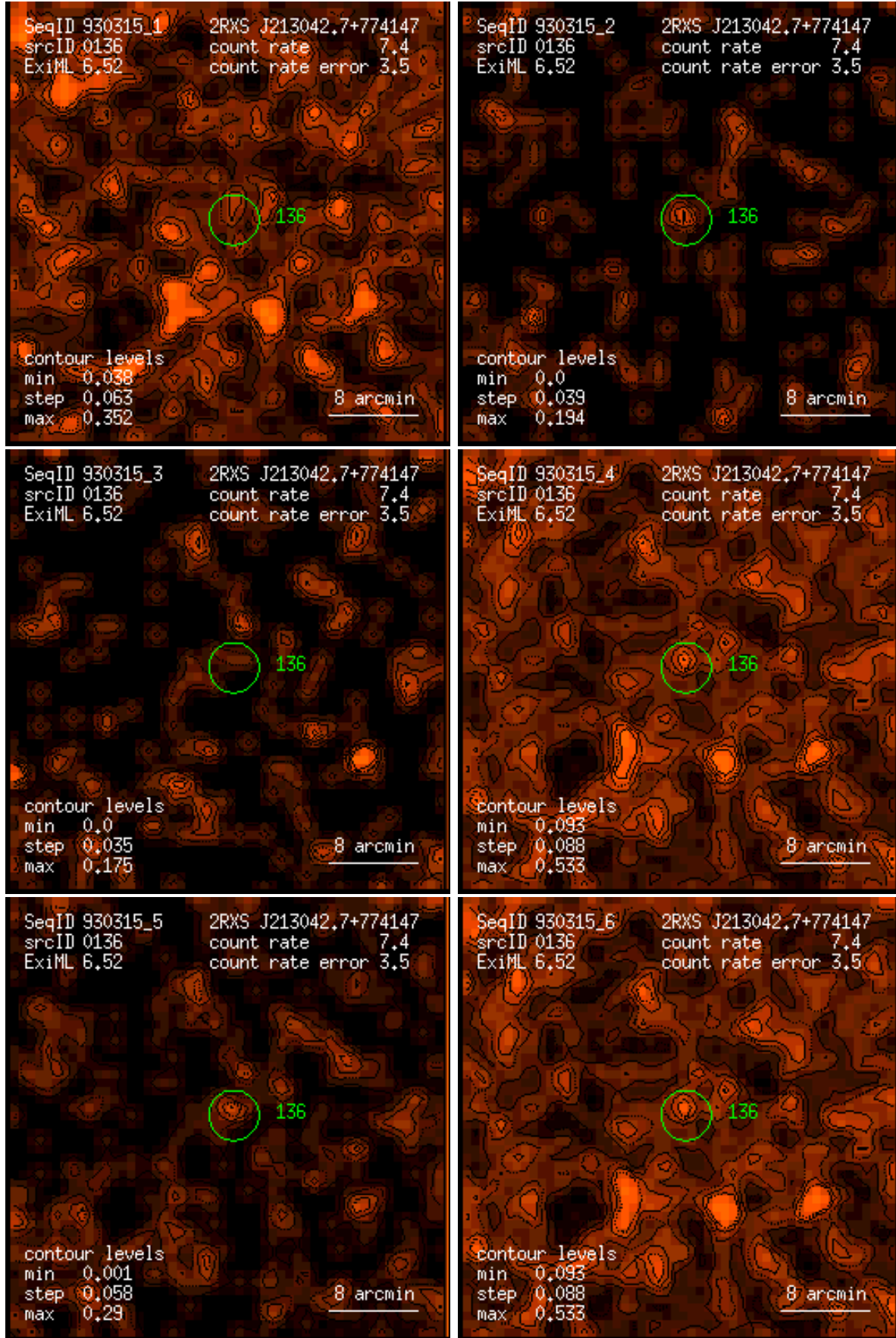
Figure 136: RASS 930315: detection 0136: band rate images, Gaussian filter: (1) PSPC channels 11 – 41, (2) 52 – 90, (3) 91 – 201, (4) 11 – 235, (5) 52 – 201, (6) 11 – 201. Broad band rates in counts/ks. Band rate contour levels in counts/ks/arcmin 2 .
