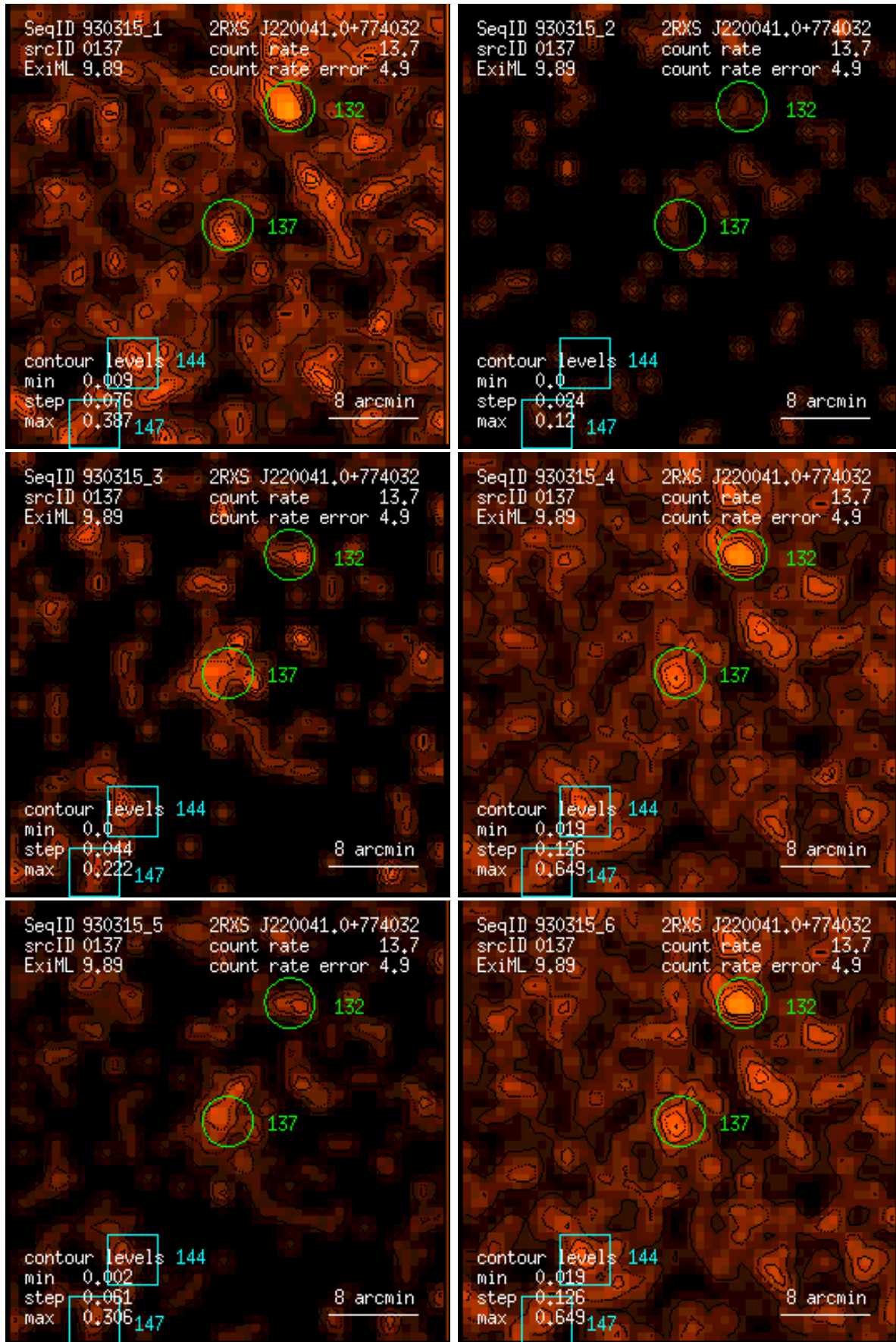
Figure 137: RASS 930315: detection 0137: band rate images, Gaussian filter: (1) PSPC channels 11 – 41, (2) 52 – 90, (3) 91 – 201, (4) 11 – 235, (5) 52 – 201, (6) 11 – 201. Broad band rates in counts/ks. Band rate contour levels in counts/ks/arcmin 2 .
