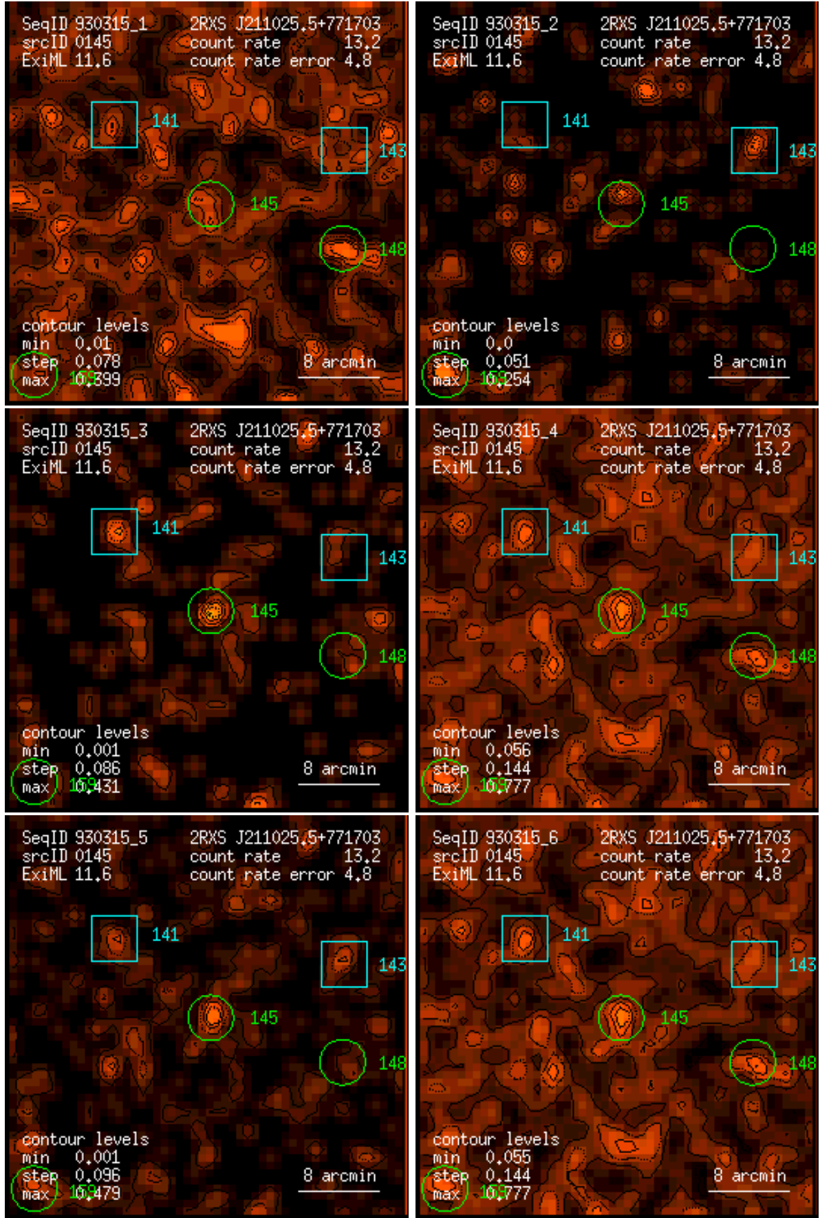
Figure 145: RASS 930315: detection 0145: band rate images, Gaussian filter: (1) PSPC channels 11 – 41, (2) 52 – 90, (3) 91 – 201, (4) 11 – 235, (5) 52 – 201, (6) 11 – 201. Broad band rates in counts/ks. Band rate contour levels in counts/ks/arcmin 2 .
