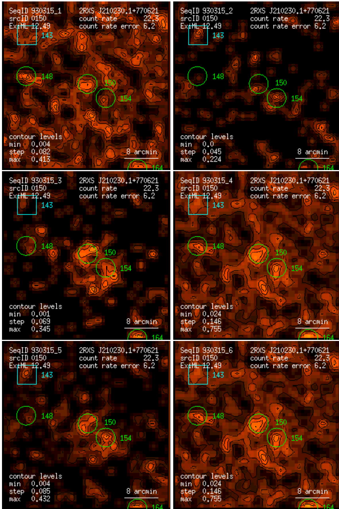
Figure 150: RASS 930315: detection 0150: band rate images, Gaussian filter: (1) PSPC channels 11 – 41, (2) 52 – 90, (3) 91 – 201, (4) 11 – 235, (5) 52 – 201, (6) 11 – 201. Broad band rates in counts/ks. Band rate contour levels in counts/ks/arcmin 2 .
