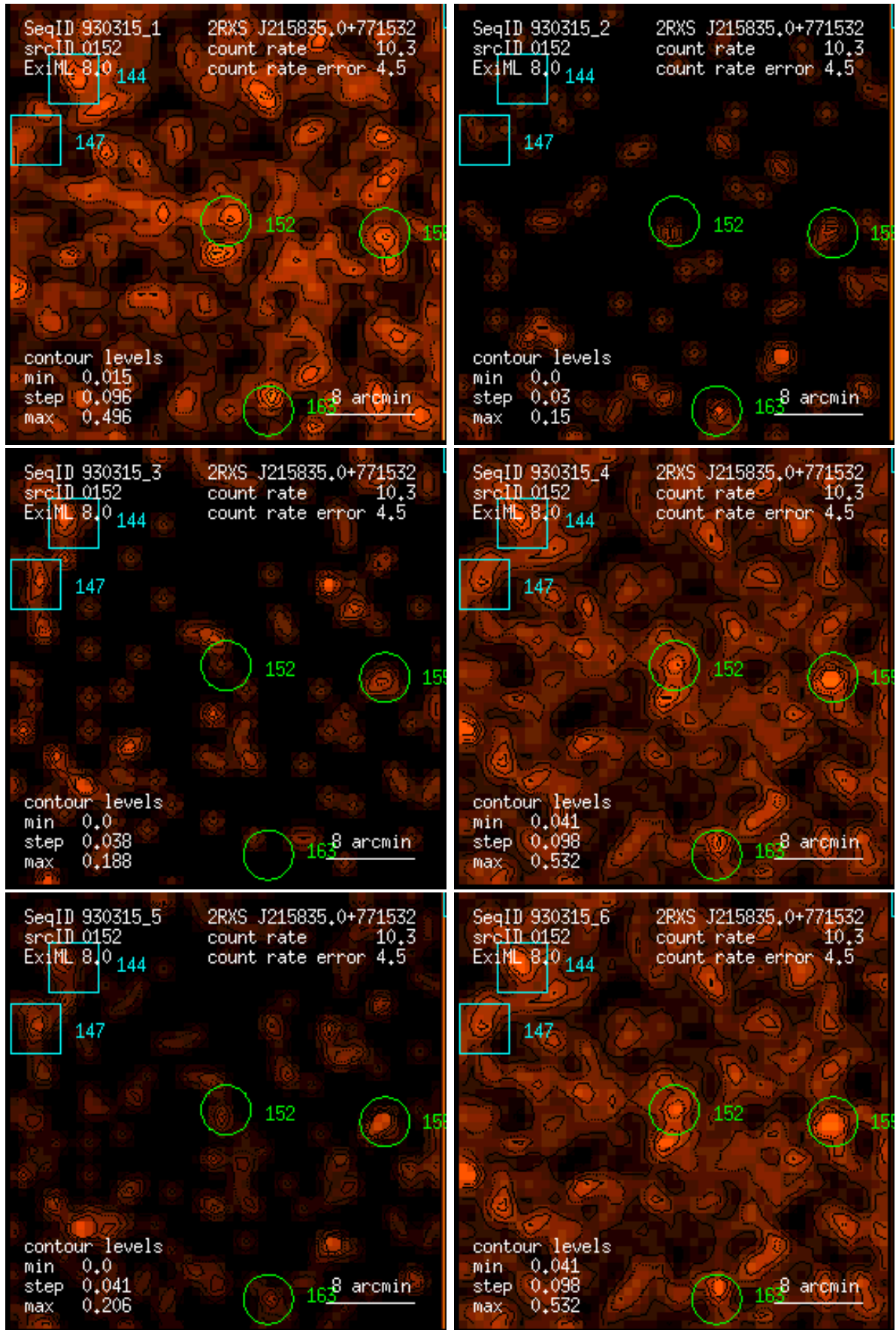
Figure 152: RASS 930315: detection 0152: band rate images, Gaussian filter: (1) PSPC channels 11 – 41, (2) 52 – 90, (3) 91 – 201, (4) 11 – 235, (5) 52 – 201, (6) 11 – 201. Broad band rates in counts/ks. Band rate contour levels in counts/ks/arcmin 2 .
