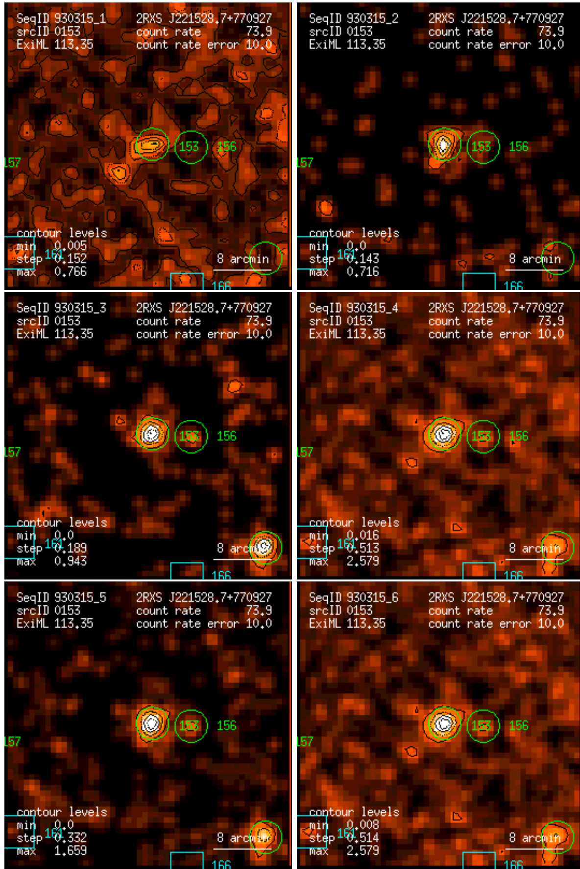
Figure 153: RASS 930315: detection 0153: band rate images, Gaussian filter: (1) PSPC channels 11 – 41, (2) 52 – 90, (3) 91 – 201, (4) 11 – 235, (5) 52 – 201, (6) 11 – 201. Broad band rates in counts/ks. Band rate contour levels in counts/ks/arcmin 2 .
