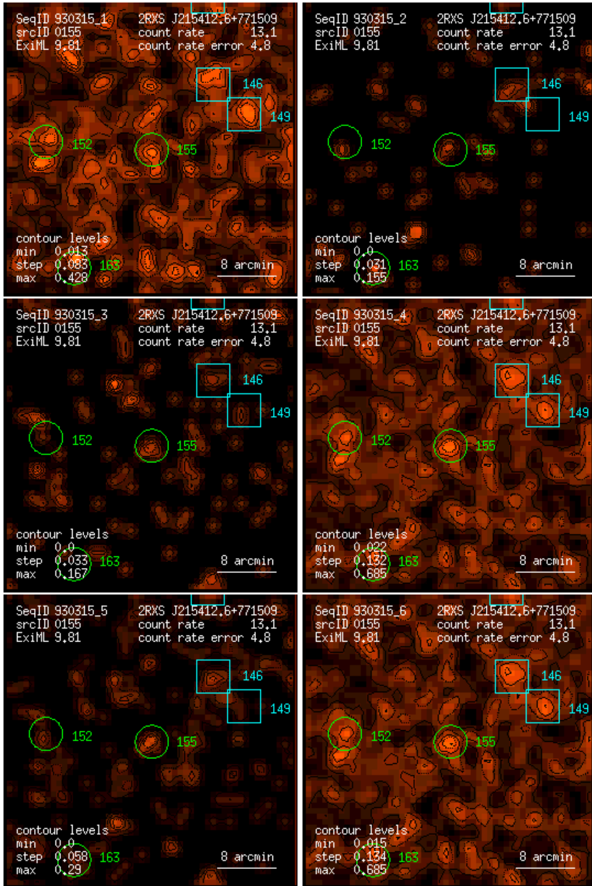
Figure 155: RASS 930315: detection 0155: band rate images, Gaussian filter: (1) PSPC channels 11 – 41, (2) 52 – 90, (3) 91 – 201, (4) 11 – 235, (5) 52 – 201, (6) 11 – 201. Broad band rates in counts/ks. Band rate contour levels in counts/ks/arcmin 2 .
