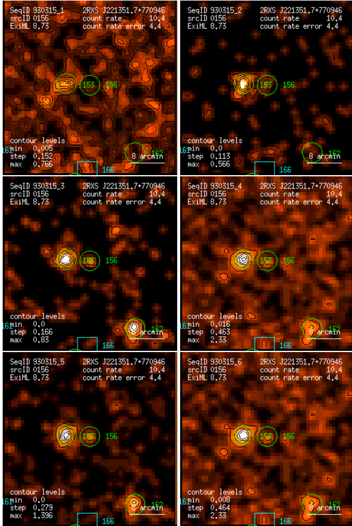
Figure 156: RASS 930315: detection 0156: band rate images, Gaussian filter: (1) PSPC channels 11 – 41, (2) 52 – 90, (3) 91 – 201, (4) 11 – 235, (5) 52 – 201, (6) 11 – 201. Broad band rates in counts/ks. Band rate contour levels in counts/ks/arcmin 2 .
