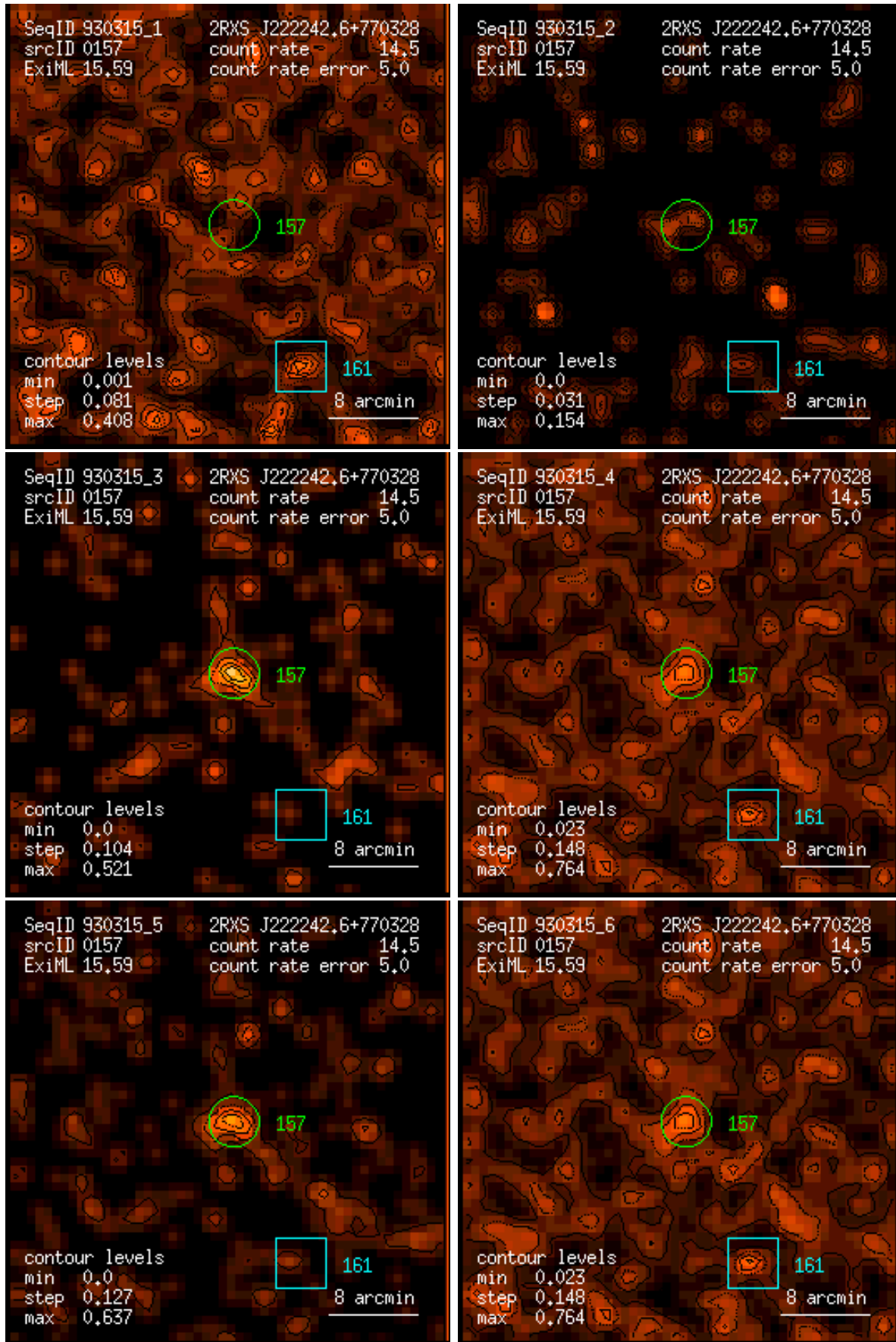
Figure 157: RASS 930315: detection 0157: band rate images, Gaussian filter: (1) PSPC channels 11 – 41, (2) 52 – 90, (3) 91 – 201, (4) 11 – 235, (5) 52 – 201, (6) 11 – 201. Broad band rates in counts/ks. Band rate contour levels in counts/ks/arcmin 2 .
