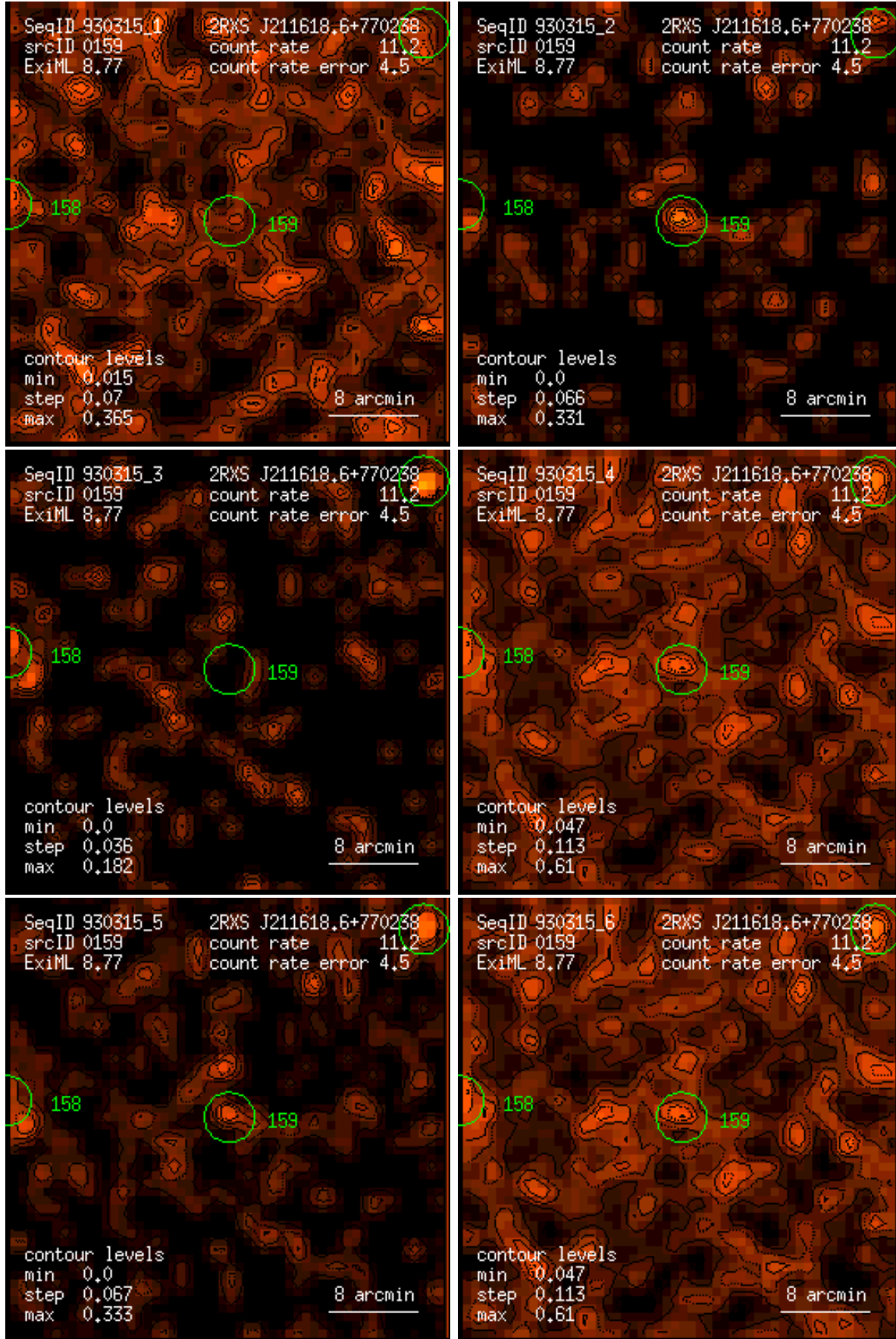
Figure 159: RASS 930315: detection 0159: band rate images, Gaussian filter: (1) PSPC channels 11 – 41, (2) 52 – 90, (3) 91 – 201, (4) 11 – 235, (5) 52 – 201, (6) 11 – 201. Broad band rates in counts/ks. Band rate contour levels in counts/ks/arcmin 2 .
