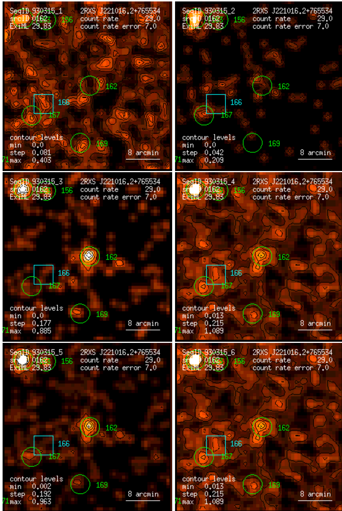
Figure 162: RASS 930315: detection 0162: band rate images, Gaussian filter: (1) PSPC channels 11 – 41, (2) 52 – 90, (3) 91 – 201, (4) 11 – 235, (5) 52 – 201, (6) 11 – 201. Broad band rates in counts/ks. Band rate contour levels in counts/ks/arcmin 2 .
