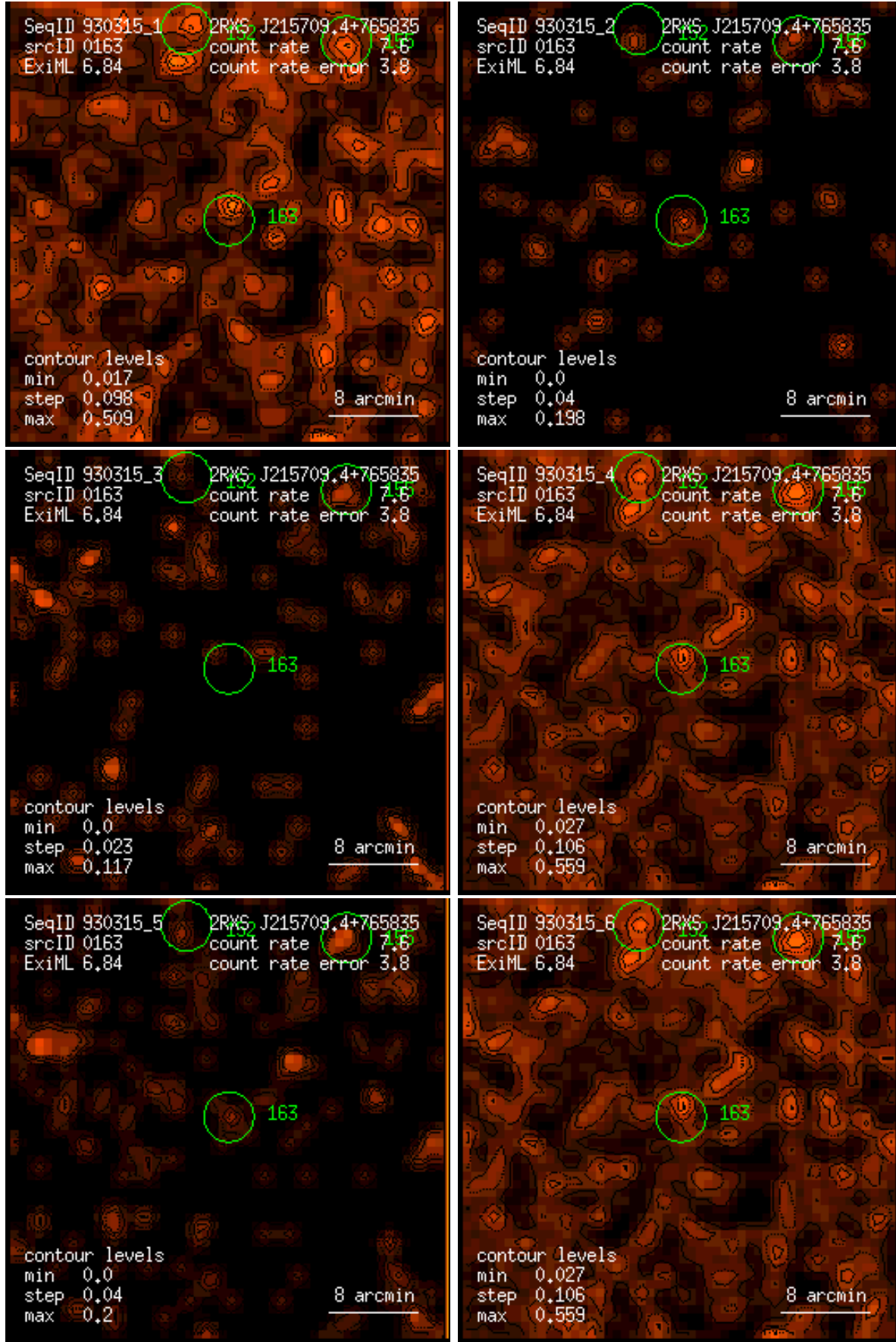
Figure 163: RASS 930315: detection 0163: band rate images, Gaussian filter: (1) PSPC channels 11 – 41, (2) 52 – 90, (3) 91 – 201, (4) 11 – 235, (5) 52 – 201, (6) 11 – 201. Broad band rates in counts/ks. Band rate contour levels in counts/ks/arcmin 2 .
