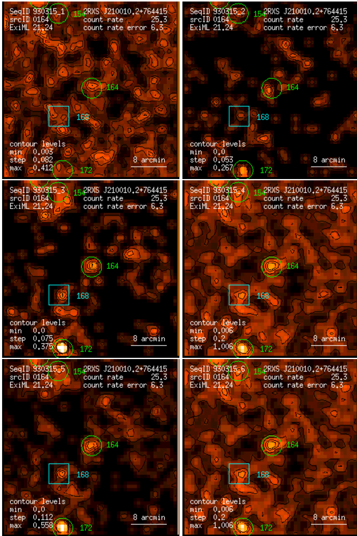
Figure 164: RASS 930315: detection 0164: band rate images, Gaussian filter: (1) PSPC channels 11 – 41, (2) 52 – 90, (3) 91 – 201, (4) 11 – 235, (5) 52 – 201, (6) 11 – 201. Broad band rates in counts/ks. Band rate contour levels in counts/ks/arcmin 2 .
