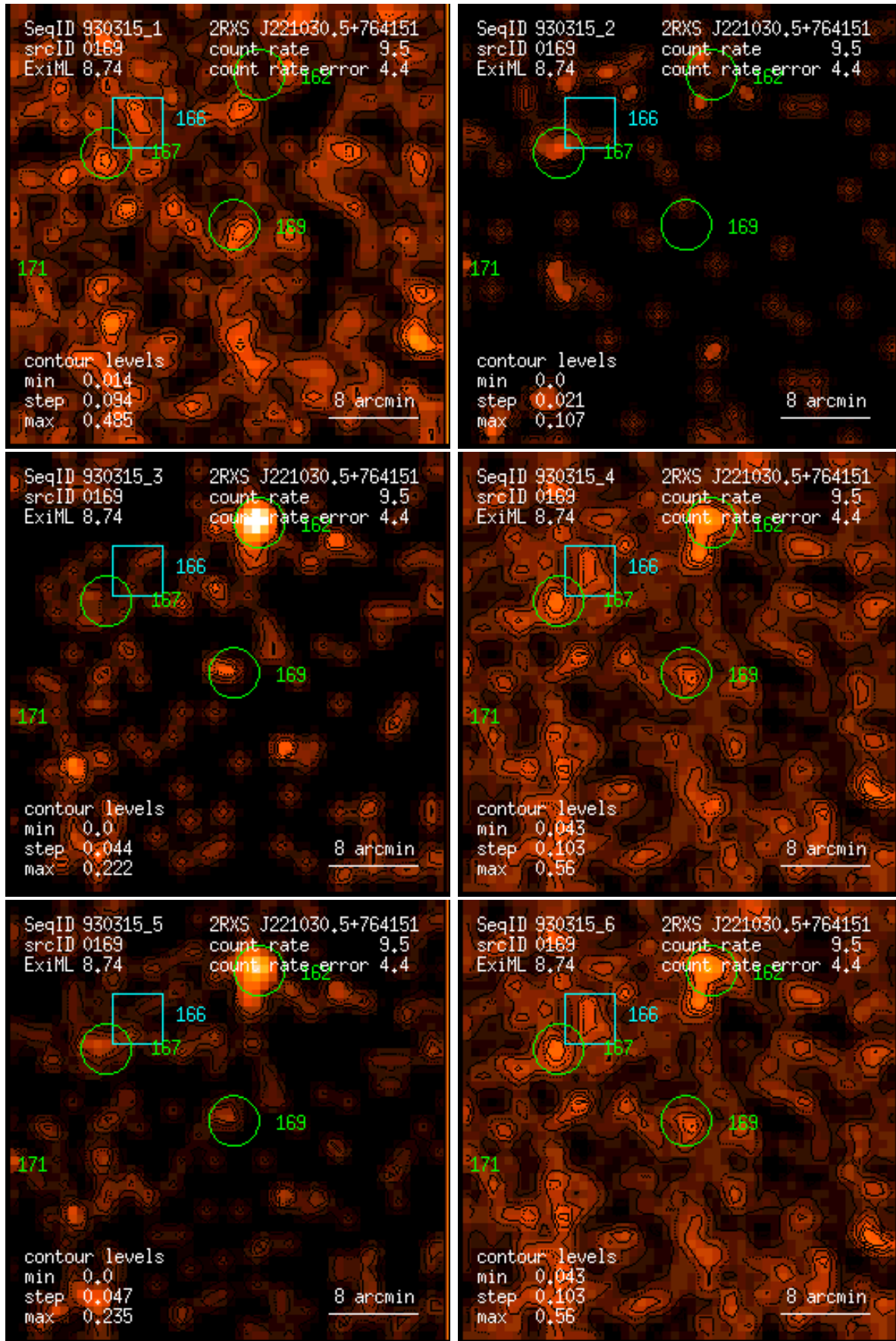
Figure 169: RASS 930315: detection 0169: band rate images, Gaussian filter: (1) PSPC channels 11 – 41, (2) 52 – 90, (3) 91 – 201, (4) 11 – 235, (5) 52 – 201, (6) 11 – 201. Broad band rates in counts/ks. Band rate contour levels in counts/ks/arcmin 2 .
