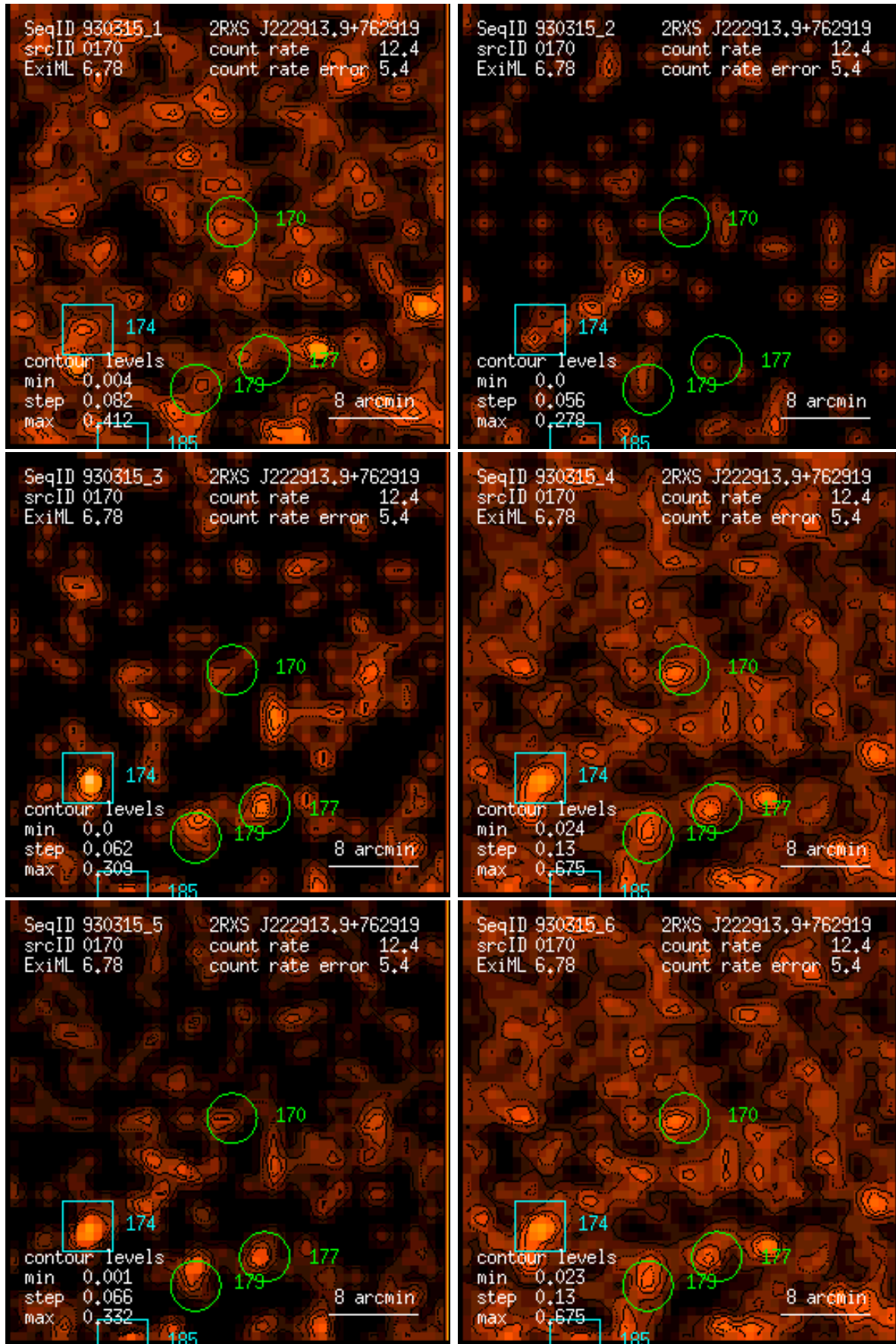
Figure 170: RASS 930315: detection 0170: band rate images, Gaussian filter: (1) PSPC channels 11 – 41, (2) 52 – 90, (3) 91 – 201, (4) 11 – 235, (5) 52 – 201, (6) 11 – 201. Broad band rates in counts/ks. Band rate contour levels in counts/ks/arcmin 2 .
