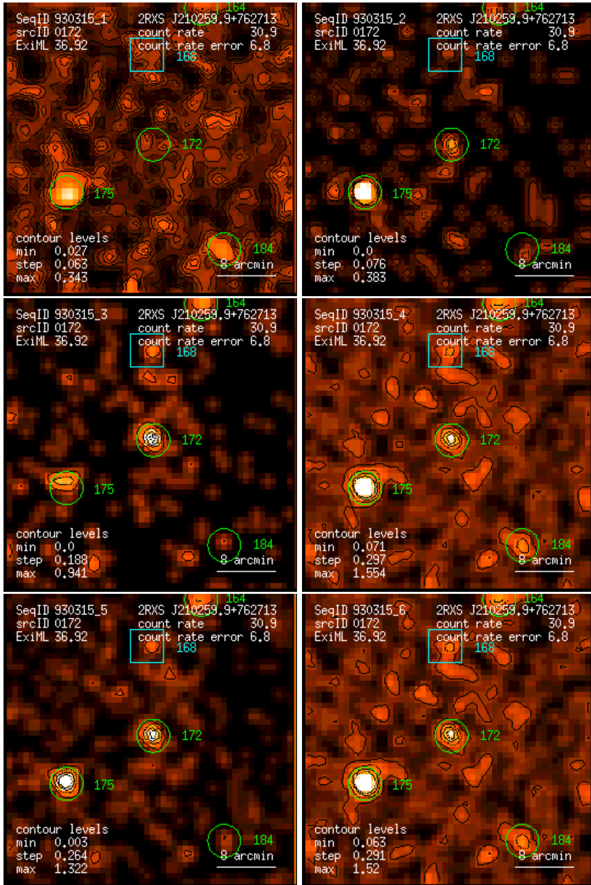
Figure 172: RASS 930315: detection 0172: band rate images, Gaussian filter: (1) PSPC channels 11 – 41, (2) 52 – 90, (3) 91 – 201, (4) 11 – 235, (5) 52 – 201, (6) 11 – 201. Broad band rates in counts/ks. Band rate contour levels in counts/ks/arcmin 2 .
