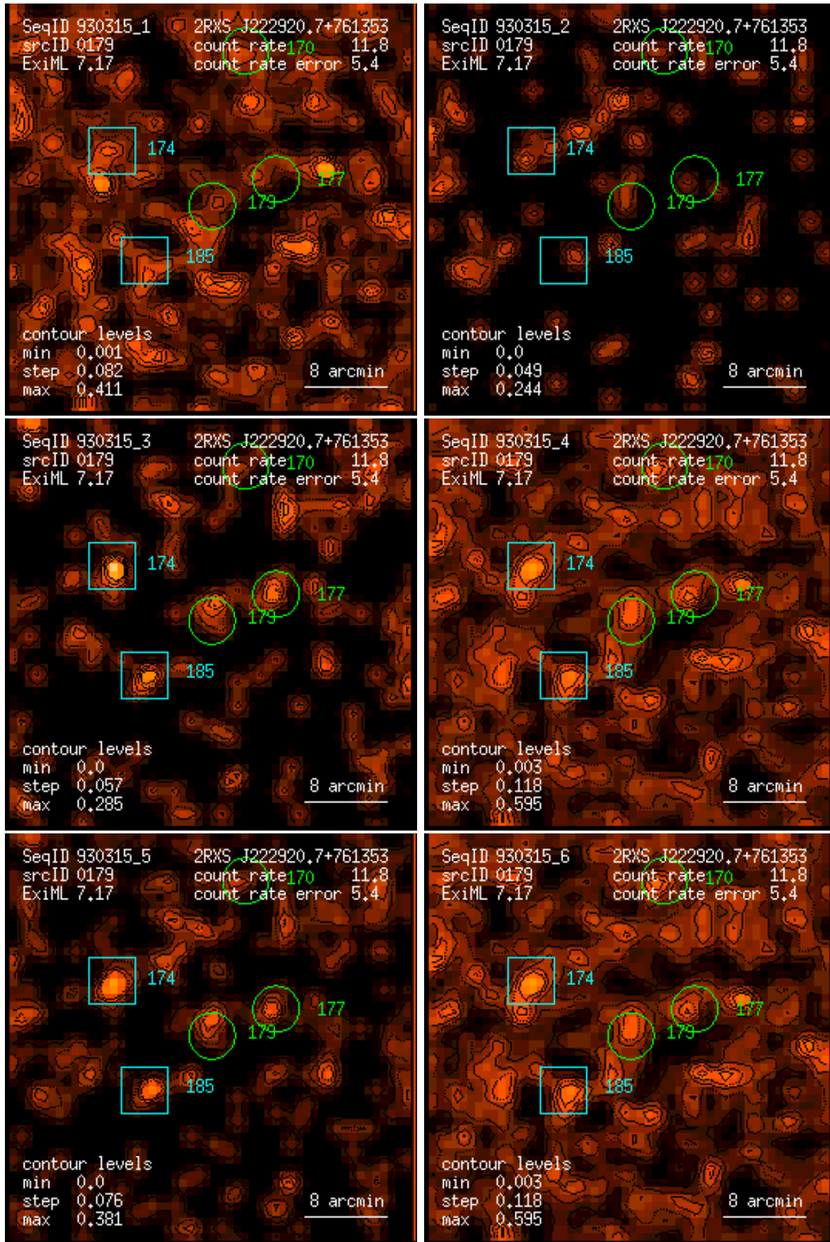
Figure 179: RASS 930315: detection 0179: band rate images, Gaussian filter: (1) PSPC channels 11 – 41, (2) 52 – 90, (3) 91 – 201, (4) 11 – 235, (5) 52 – 201, (6) 11 – 201. Broad band rates in counts/ks. Band rate contour levels in counts/ks/arcmin 2 .
