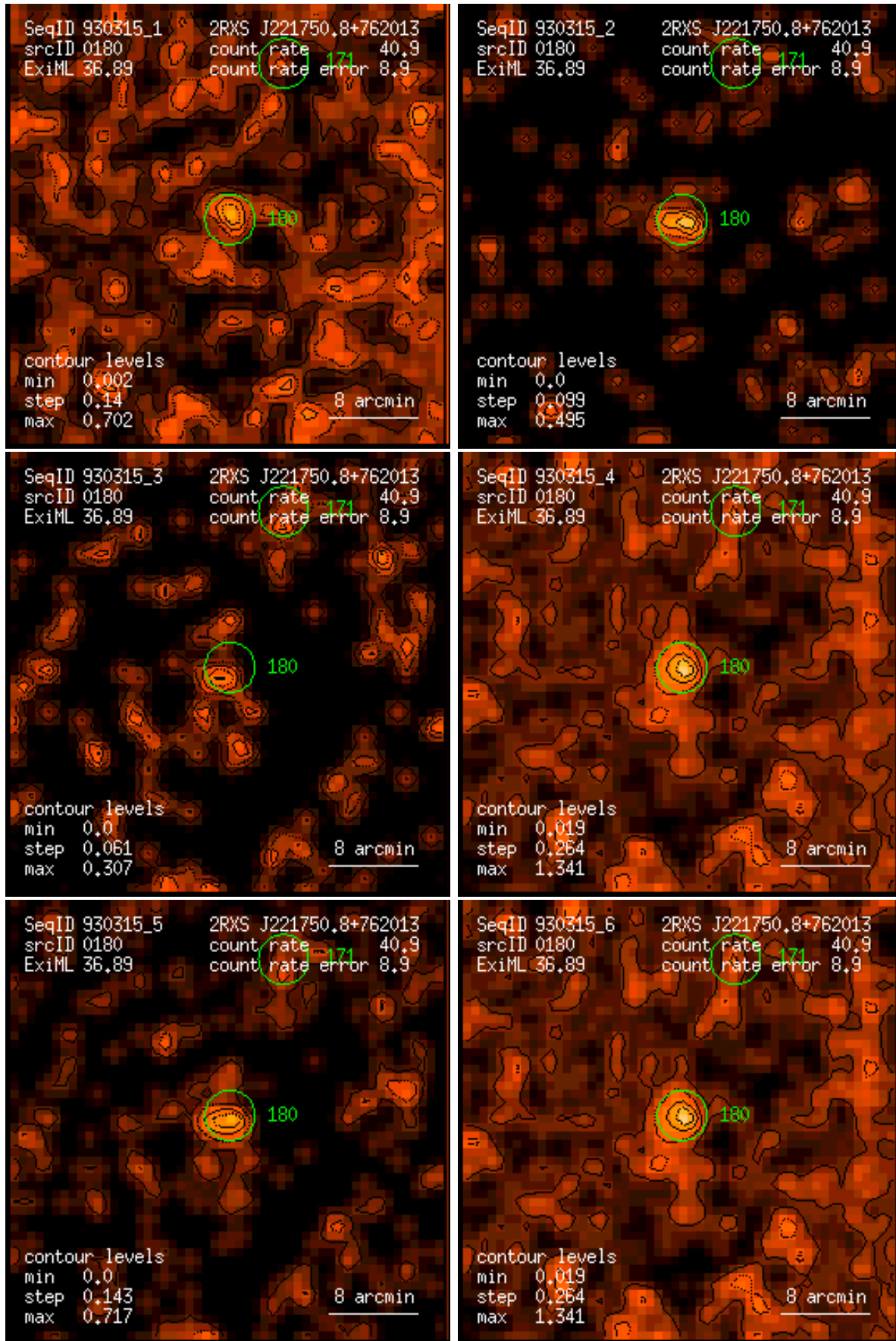
Figure 180: RASS 930315: detection 0180: band rate images, Gaussian filter: (1) PSPC channels 11 – 41, (2) 52 – 90, (3) 91 – 201, (4) 11 – 235, (5) 52 – 201, (6) 11 – 201. Broad band rates in counts/ks. Band rate contour levels in counts/ks/arcmin 2 .
